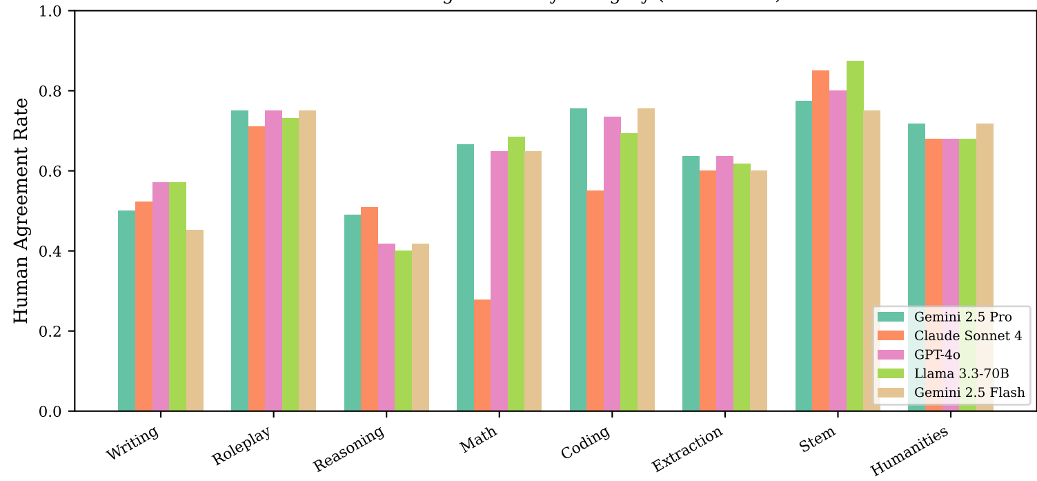
MT-Bench Agreement by Category (B0 Baseline)
