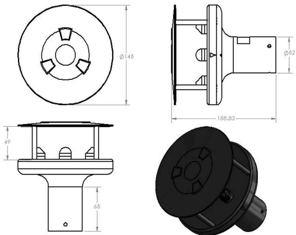
Ultrasonic Anemometer (all dimensions are in mm)
