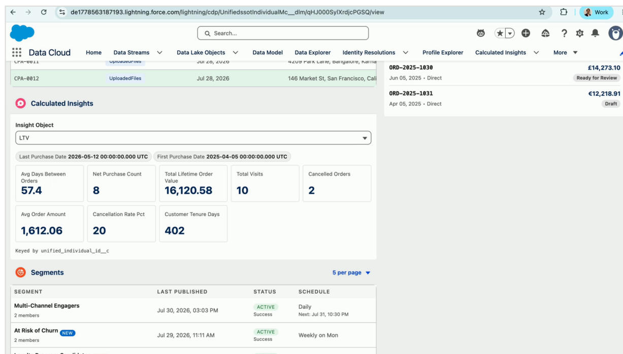
Figure 5 — Calculated insight measures for this profile, and the segments it belongs to with publish status and schedule.
