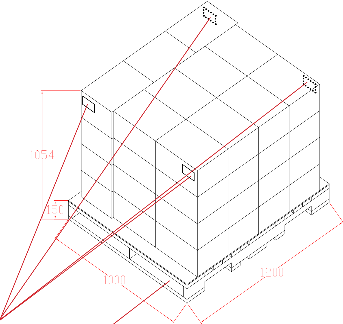
VIEW D PALLET LABEL Shared usage with the carton label.
