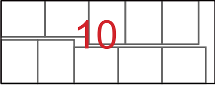
20" Container ( 1200x1000 pallet )
