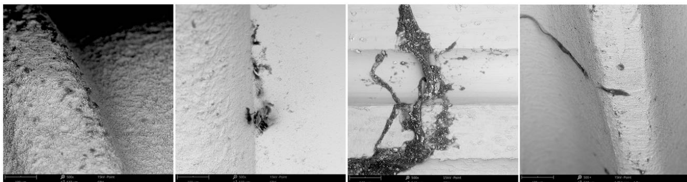
SEM images revealing significant amounts of carbonaceous particles on new, sterile packaged dental implants
