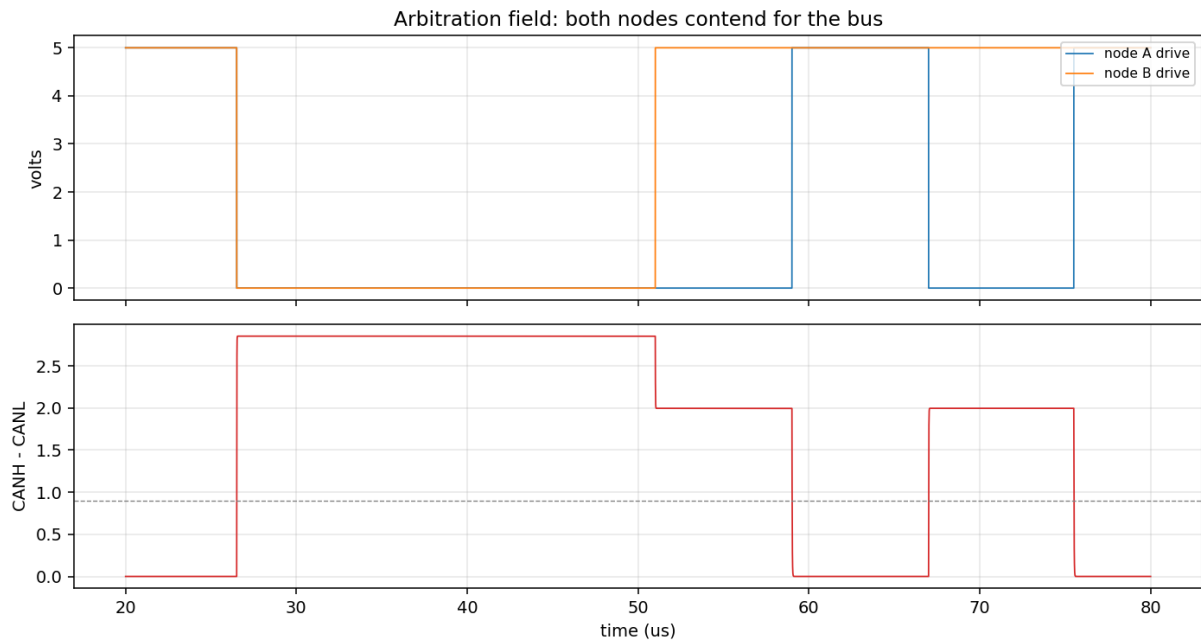
Figure 3. Arbitration field. Both nodes drive the bus; the elevated differential indicates simultaneous dominant drive.
