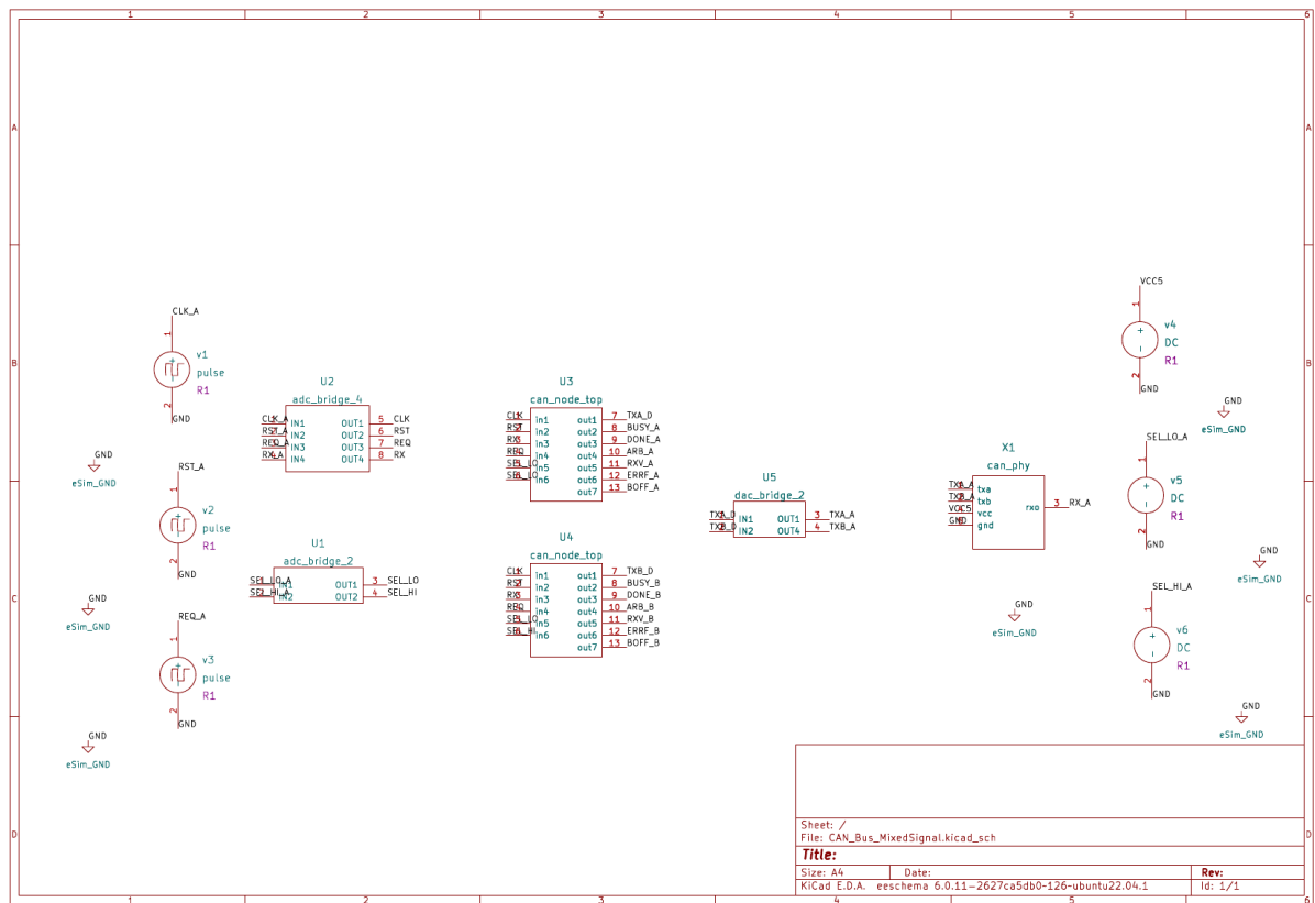
Figure 1. eSim schematic. Two can_node_top NGHDL controllers (U3, U4) share the can_phy transceiver subcircuit (X1). Bridges U1 and U2 convert the analog stimulus to the digital domain and U5 returns the transmit outputs to analog.
