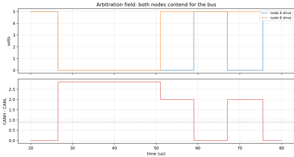
Figure 3. Arbitration field. Both nodes drive the bus; the elevated differential indicates simultaneous dominant drive.
