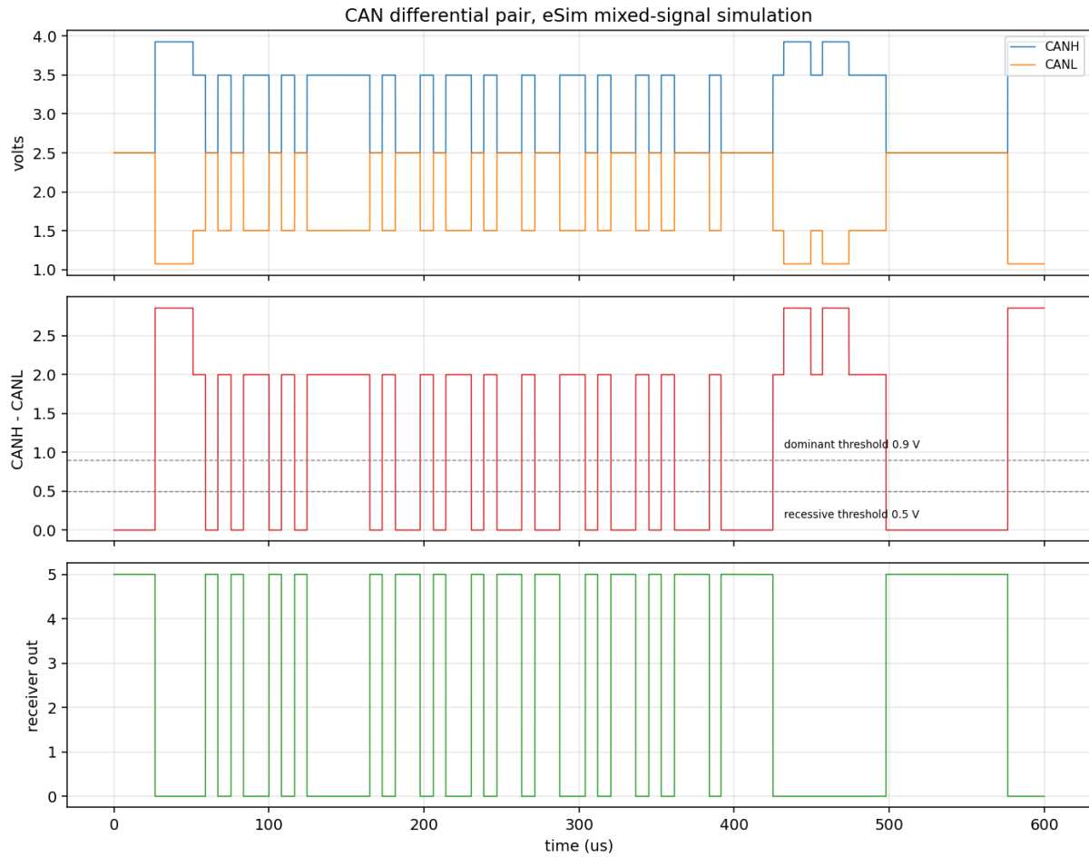
Figure 2. Complete frame. CANH and CANL (top), differential with the ISO thresholds marked (middle), receiver output (bottom).
