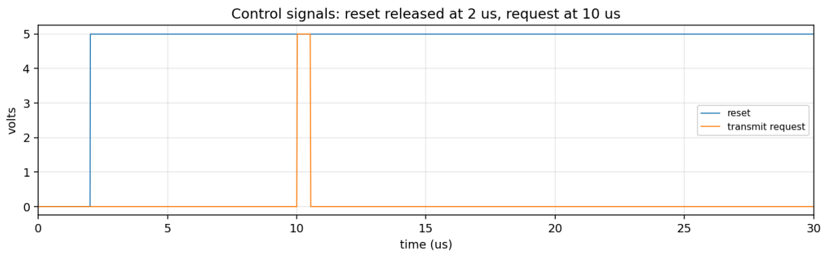
Figure 4. Control signals. Reset released at 2 us, transmit request asserted at 10 us.
