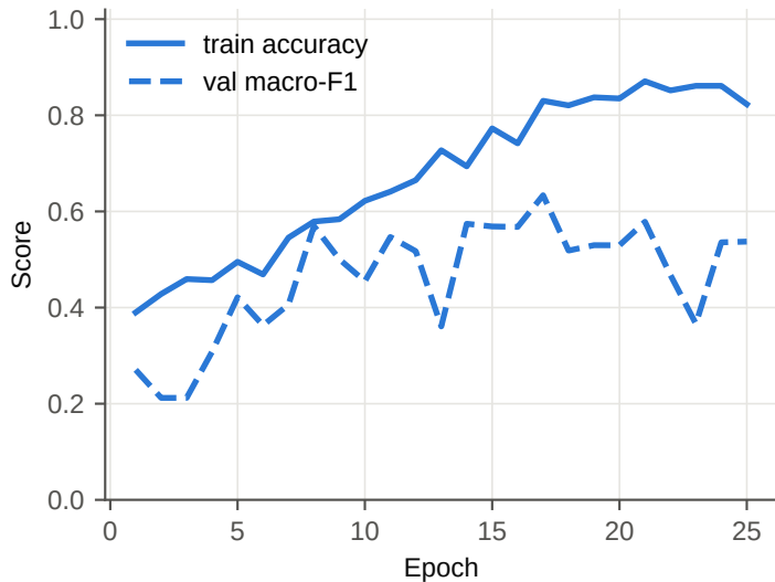
Multi-kernel CNN (emb=glove,cw=none, seed 42)
