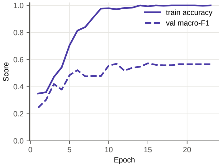
BiLSTM (emb=random,cw=bal, seed 42)
