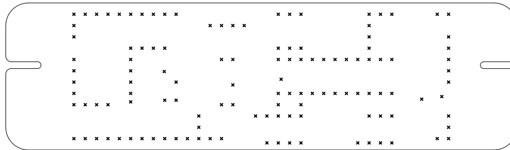
Drill Map: x 0.200mm / 0.0079" (124 holes)
