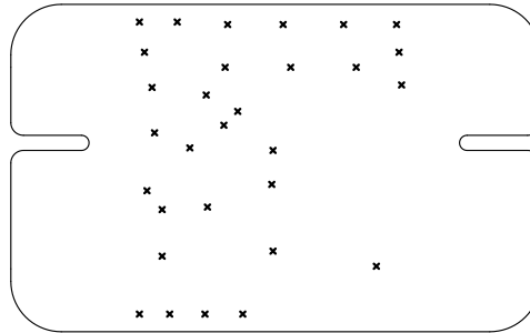
Drill Map: x 0.200mm / 0.0079" (30 holes)
