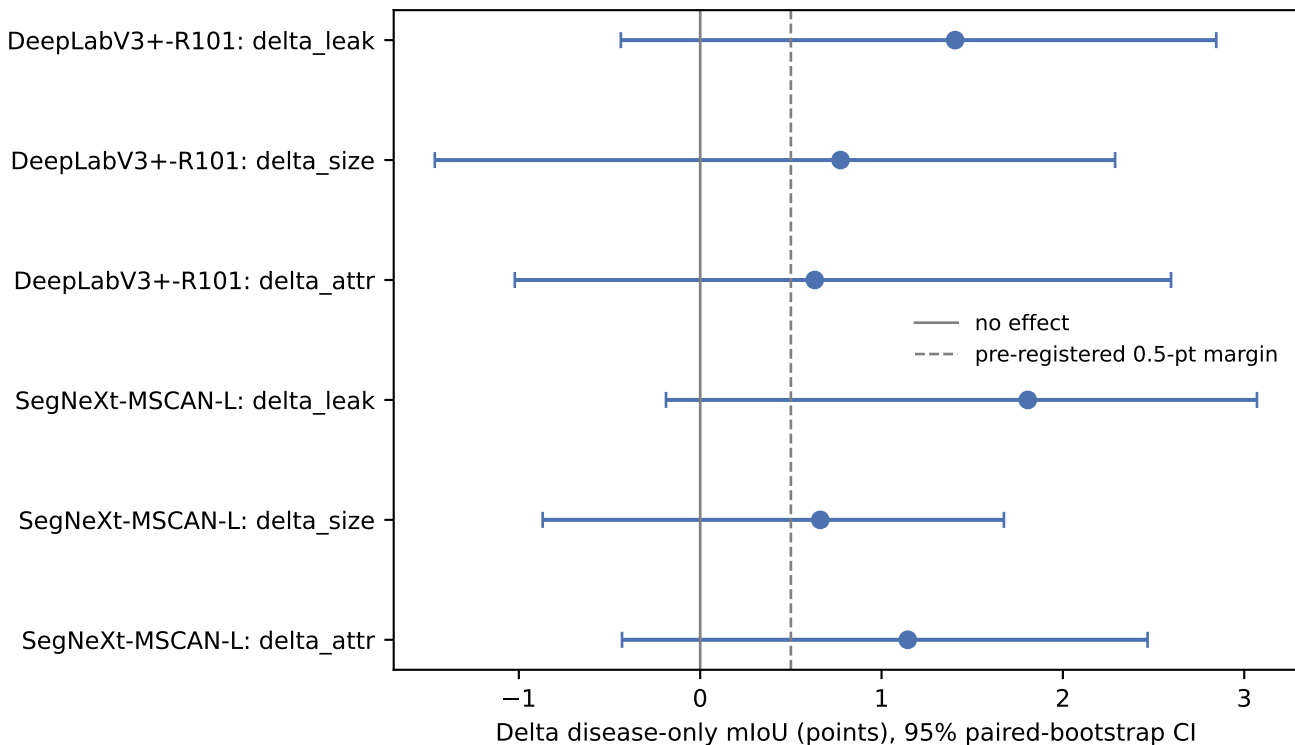
Paired effect of leakage sanitization on disease-only mIoU (fixed n=1557)
