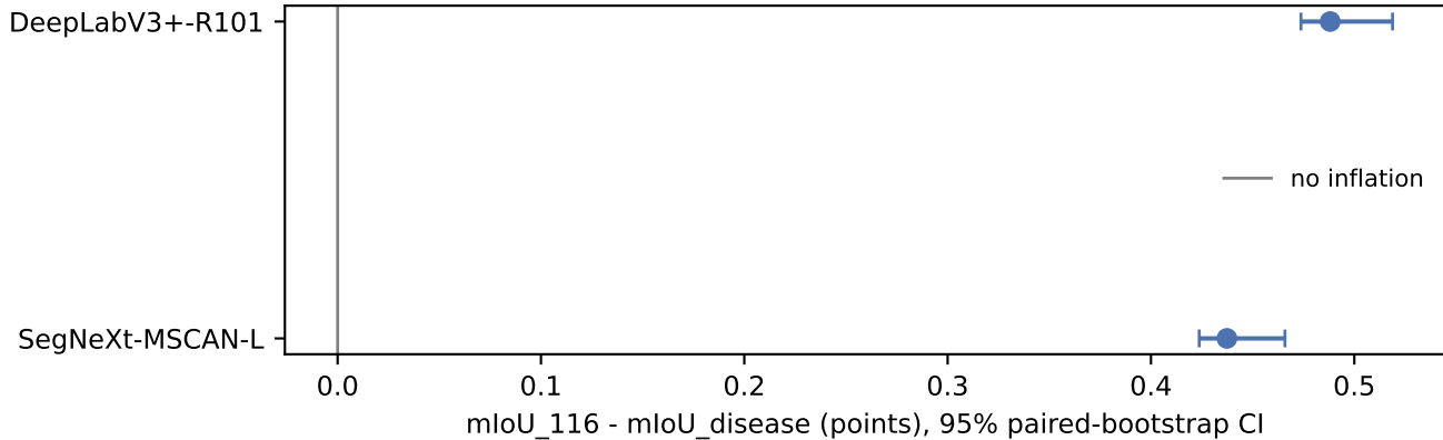
Background inclusion in the released 116-label metric (DEFAULT arm)
