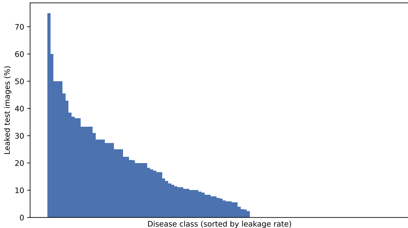
Per-class share of test images with hard cross-split near-duplicates
