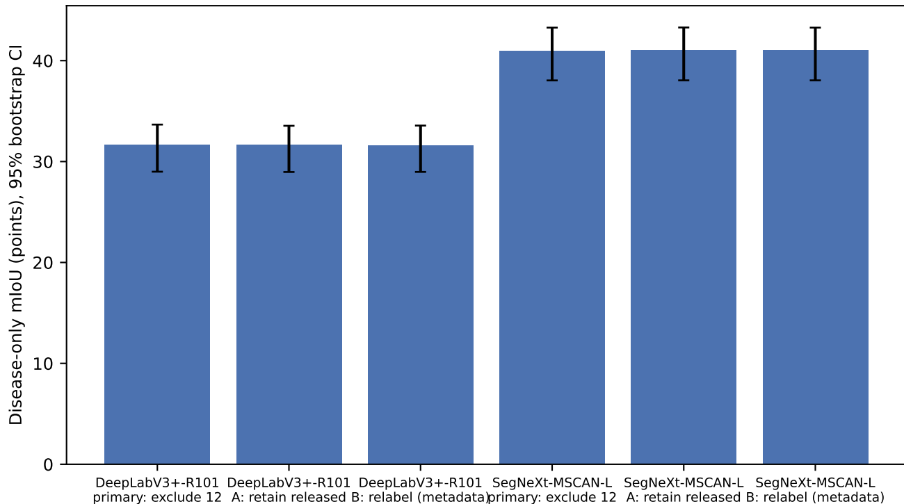
Sensitivity to the defective-mask policy (ASR-006; not claim-supporting)
