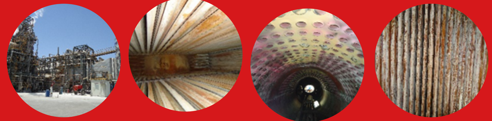
Technological Center of the Academy of Sciences of Turkmenistan – Assessment of the technical condition of a waste incineration boiler.
