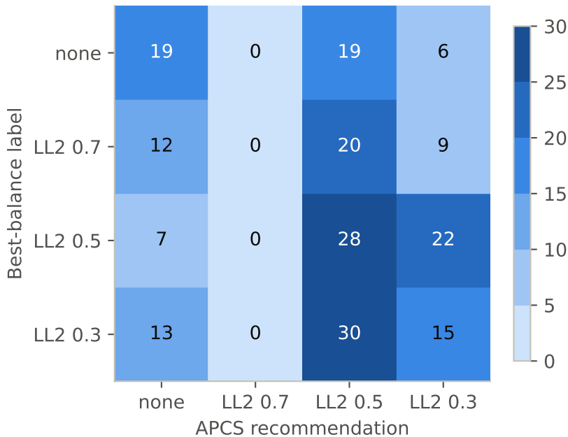
APCS confusion matrix (test)
