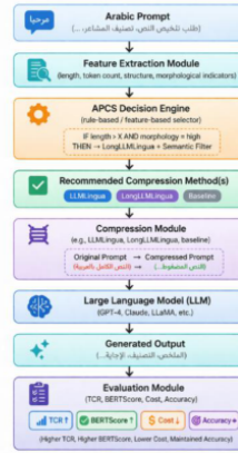
Figure 1. Architecture of the Arabic-Aware Prompt Compression Selector (APCS)
