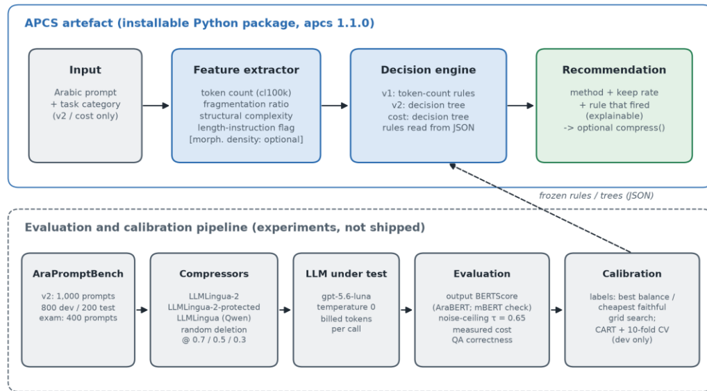
Figure 1. Architecture of the APCS artefact and the evaluation pipeline that calibrates it
