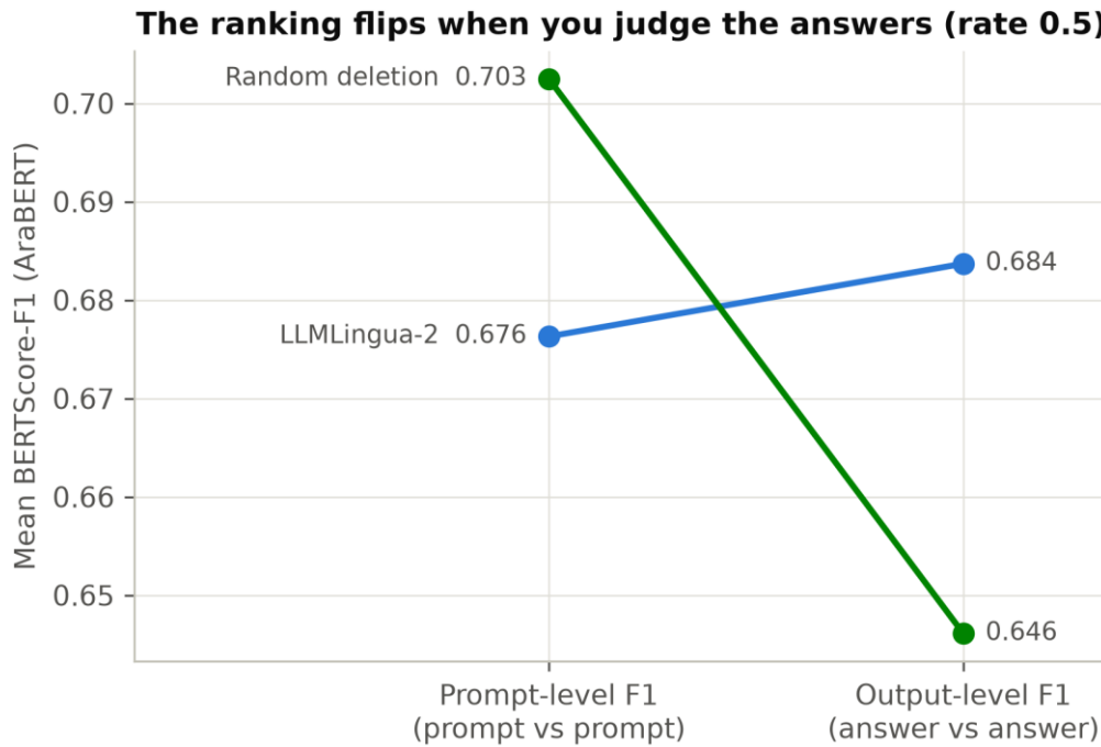
Figure 4. The ranking flip: LLMLingua-2 minus random deletion at prompt level (negative) and output level (positive)
