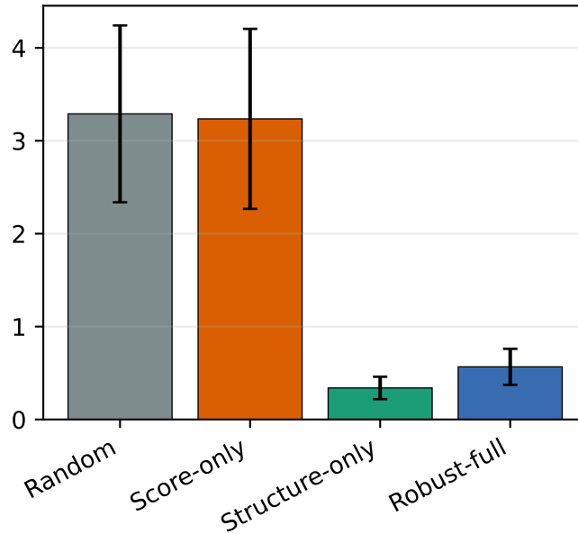
|\Delta\text{MFE}| (kcal/mol) (lower is better)
