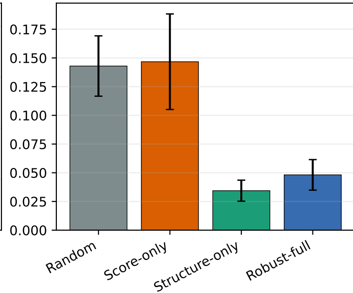
Pairing-profile L_1 (lower is better)
