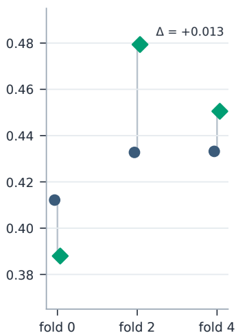
MCC
