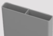
2 90x16.5mm slat with centre web 6100mm long QS-6100-S90
