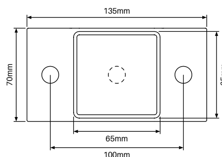
BOTTOM ANCHOR DETAIL
