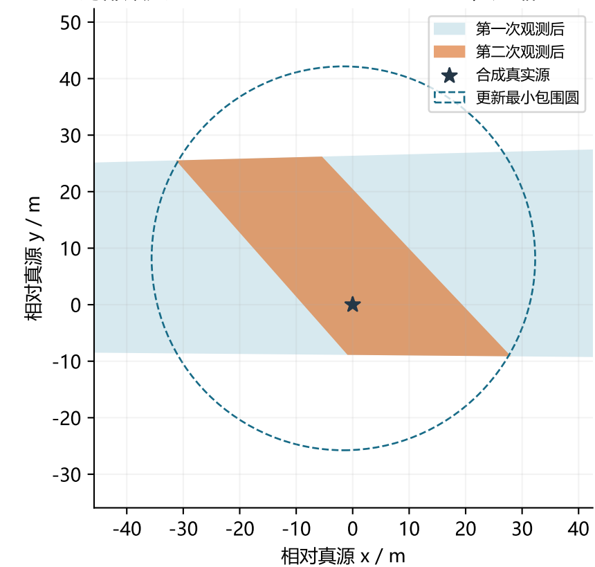
局部放大：R1=750.3 m → R2=34.0 m；压缩 95.5%
