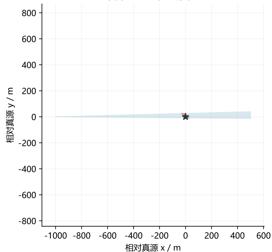
局部放大：R1=750.3 m → R2=34.0 m；压缩 95.5%
