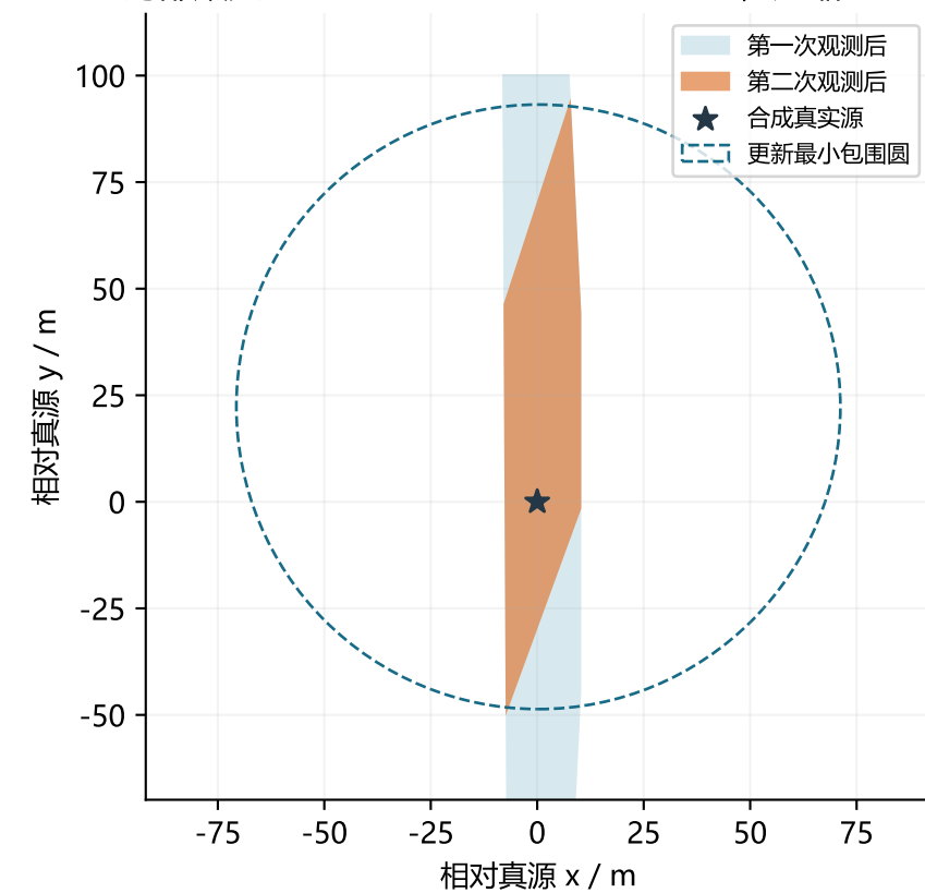
局部放大：R1=170.7 m → R2=70.9 m；压缩 58.5%
