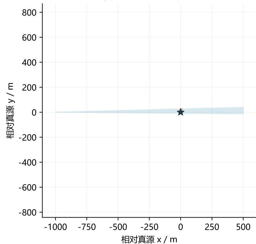
局部放大：R1=750.3 m \rightarrow R2=21.6 m；压缩 97.1%
