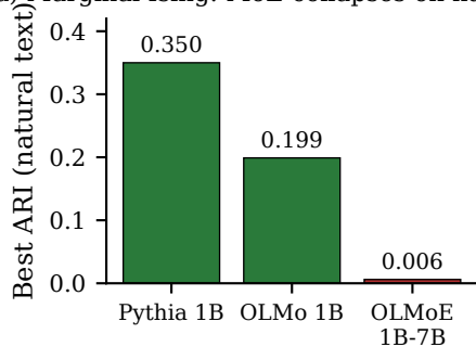
(a) Marginal Ising: MoE collapses on natural text
