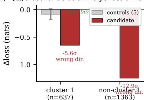
(c) Closure: ablation helps loss (wrong dir.)
