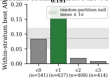
(b) Route-stratified: cluster 1 above null (+3 \sigma )
