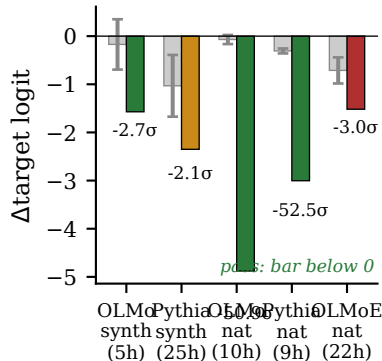
\Delta\text{target logit} ( \downarrow damage)
