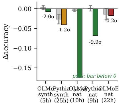
\Delta\text{accuracy} ( \downarrow damage)
