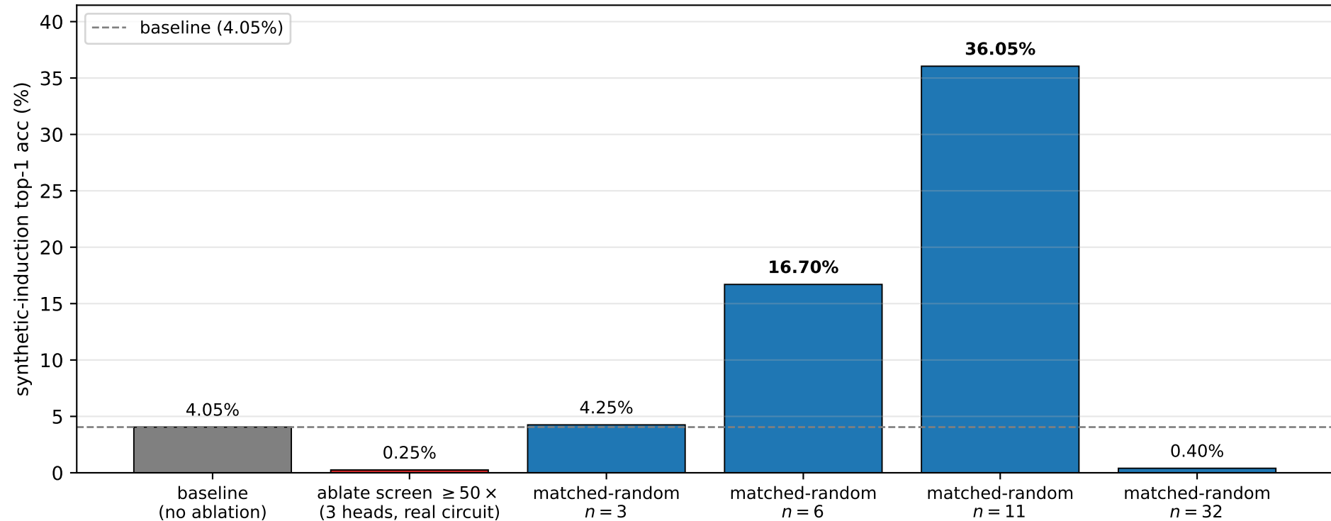
Pythia 1B: matched-random ablation of 6-11 heads in induction-circuit layers raises top-1 above baseline (BOS-attractor suppression released)
