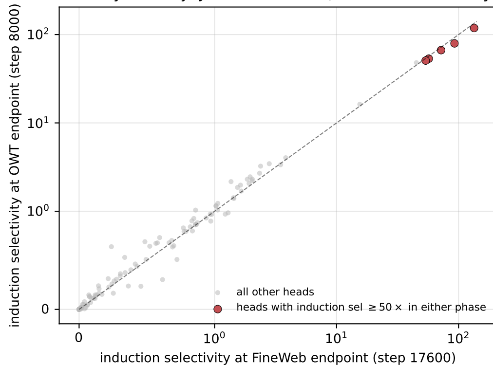
(C) Induction-circuit identity stability: Jaccard = 1.00 (shared = 5, FW-only = 0, OWT-only = 4) (D) Selectivity through OWT for FineWeb-endpoint induction heads
