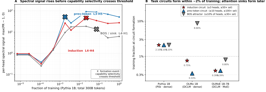
Figure 1: Capability circuits form early in pretraining and the per-head spectral signal precedes formation. Reproduced from the companion methodology paper [Anonymous, 2026a]. (A) Per-head spectral signal \max(\text{PR}_t - 1, 0) across training for three identified heads in Pythia 1B (an induction head L4·H4, a previous-token head L3·H5, a BOS-attractor head L4·H1). X markers indicate the formation event, the first revision at which the head’s capability-selectivity ratio exceeds its threshold. (B) Training fraction at circuit formation across three 1B-class configurations: capability circuits (induction, previous-token) form within the first 0.3–2.1% of training in every configuration; the BOS attractor forms later, with order-of-magnitude variation across configurations.
