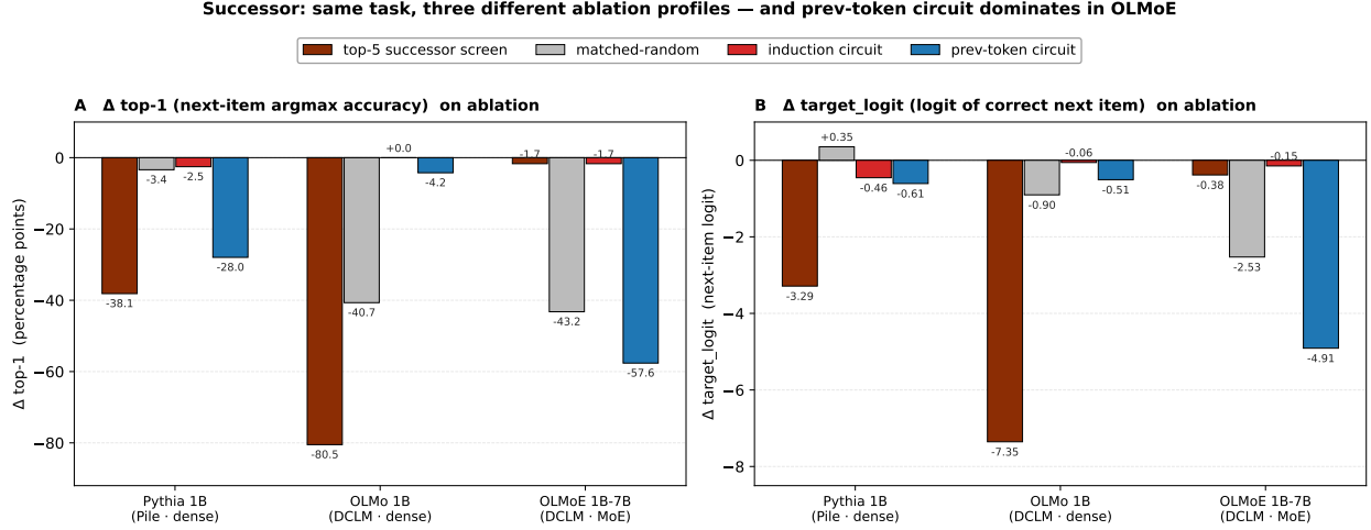
Figure 2: Successor sequences: same task, three different ablation profiles. (A) \Delta\text{top-1} ( P[\text{argmax} = \text{correct next item}] , percentage points) under each ablation. (B) \Delta\text{target\_logit} (raw logit of the correct next item). Conditions match Figure 1 except top-5 successor screen replaces top-5 GT screen . Three profiles: Pythia 1B has mixed mechanism — top-5 successor screen drops top-1 by 38.1pp and prev-token circuit drops top-1 by 28.0pp (both above matched-random \Delta -3.4); OLMo 1B ’s top-5 screen tanks top-1 by 80.5pp but matched-random in the same layers also drops it by 40.7pp because all 5 candidates are in L0 (where input-embedding processing happens); OLMoE 1B-7B ’s prev-token circuit drops top-1 by 57.6pp — far more than the top-5 successor screen’s 1.7pp drop.
