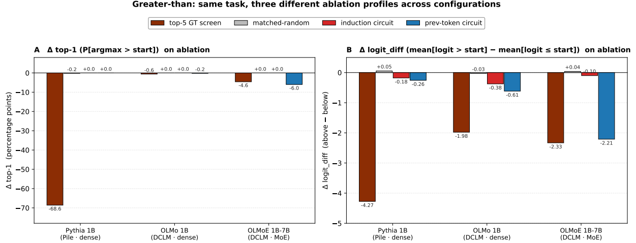
Figure 1: Greater-than: same task, three different ablation profiles across configurations. (A) \Delta \text{top-1} ( P[\text{argmax} \text{ is a 2-digit number} > \text{start}] , percentage points) on each ablation condition vs. baseline, for the three 1B-class configurations. (B) \Delta \text{logit\_diff} ( \text{mean}[\text{logit over above}] - \text{mean}[\text{logit over below}] ) on the same conditions. Conditions: top-5 GT screen (heads selected by attention from query position to start-decade position; task-specific), matched-random (5 random heads in the same layers as the top-5 GT picks, no overlap; null control), induction circuit (heads with induction selectivity \geq 50\times on the synthetic induction batch; a different screen on a different task), prev-token circuit (heads with best-class prev-token and selectivity \geq 100\times ). Three different ablation profiles emerge: Pythia 1B’s GT is concentrated in the 5 GT-specific heads ( \Delta \text{top-1} = -68.6\text{pp} ; everything else \leq 1\text{pp} ); OLMo 1B is top-1-robust to every ablation tried but the GT-screen compresses the logit margin ( \Delta \text{logit\_diff} = -1.98 with \Delta \text{top-1} only -0.6 ); OLMoE 1B-7B’s prev-token circuit ablation hurts greater-than more than the GT-specific screen does ( \Delta \text{top-1} = -6.0 vs. -4.6 ; both above the matched-random null of 0).
