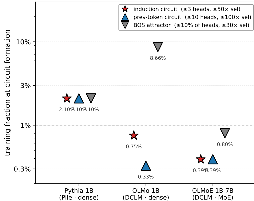
A | Spectral signal rises before capability selectivity crosses threshold B | Task circuits form within ~2% of training across configurations; attention sinks form later
