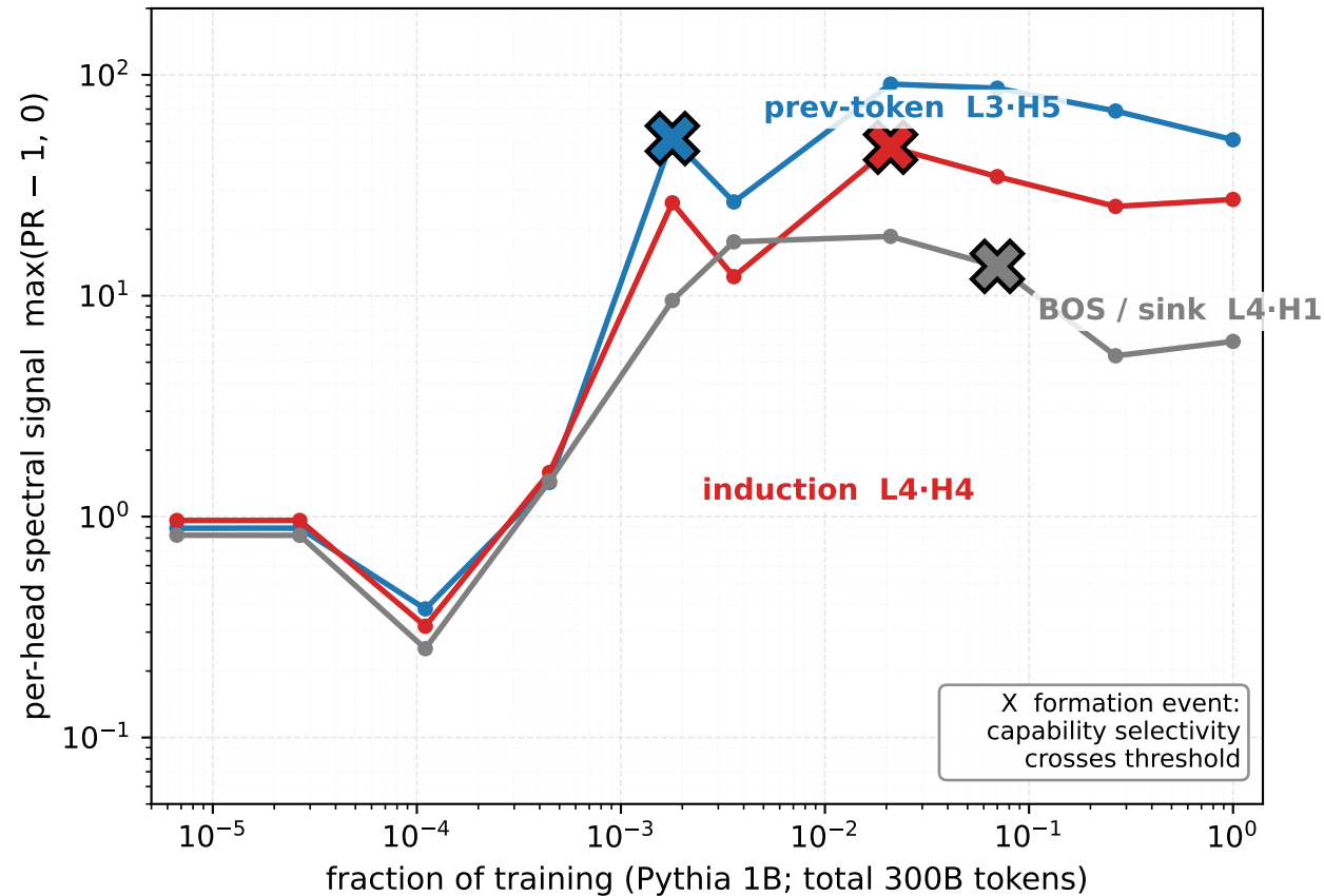
A | Spectral signal rises before capability selectivity crosses threshold B | Task circuits form within ~2% of training across configurations; attention sinks form later
