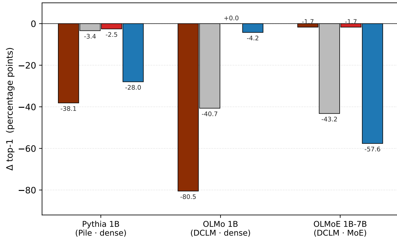
A \Delta top-1 (next-item argmax accuracy) on ablation
