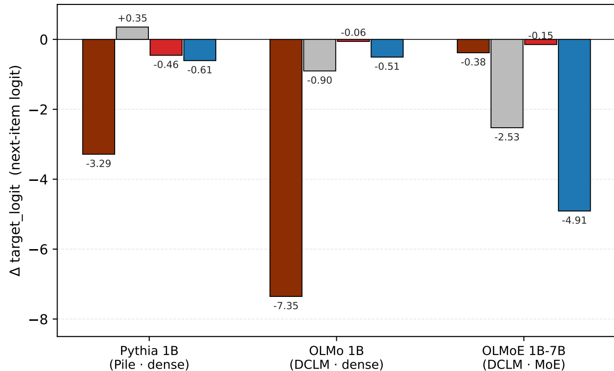
B \Delta target_logit (logit of correct next item) on ablation
