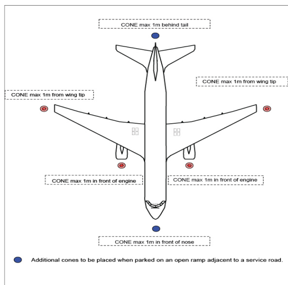
Minimum cones for a two engine aircraft
