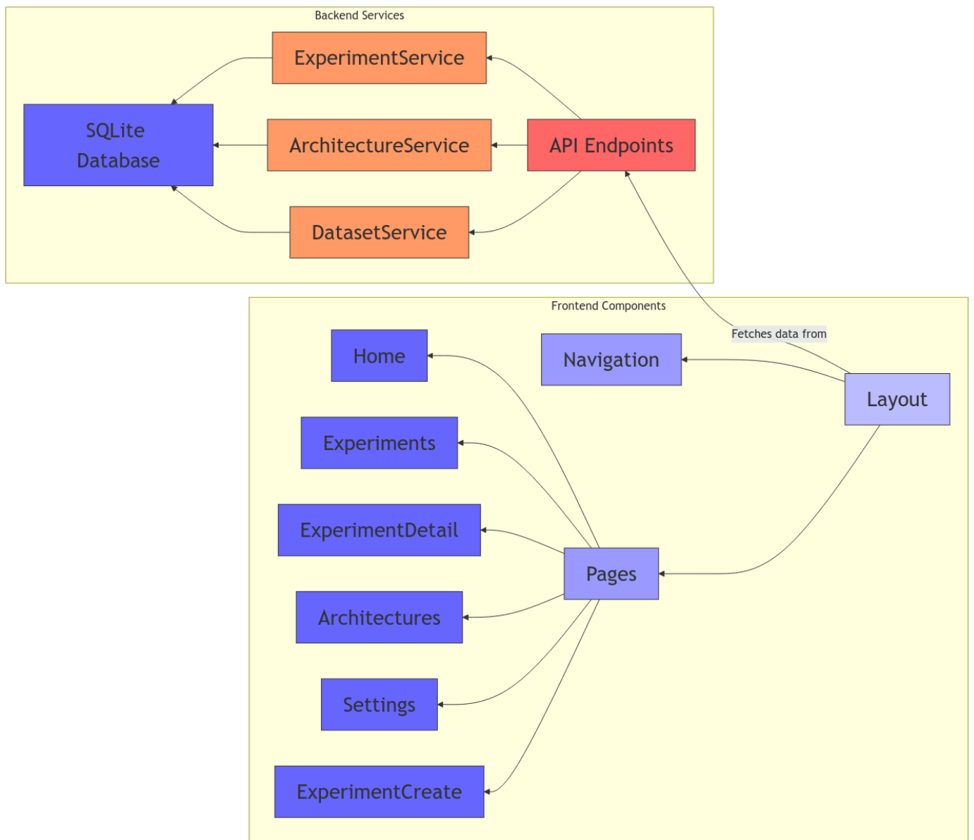
Figure 1: Component Diagram
