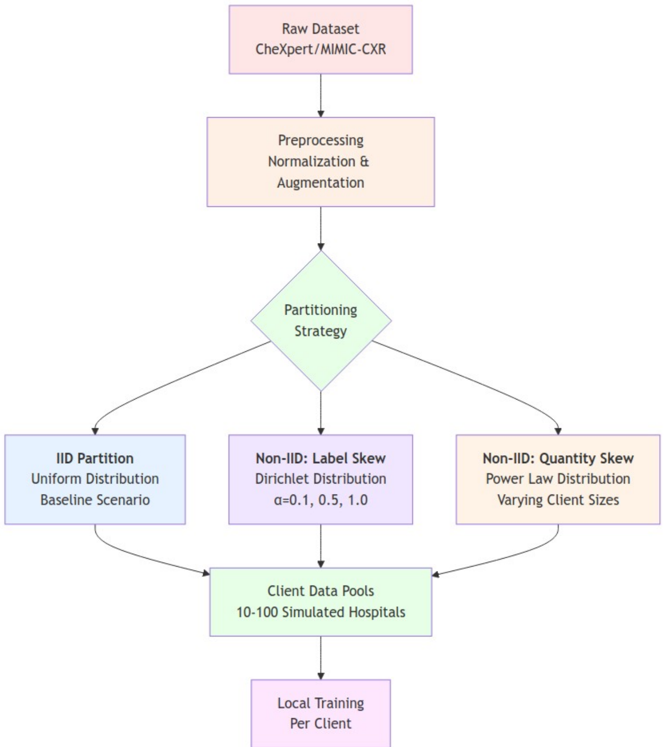
Figure 1.1: Data partitioning process
