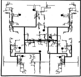
Fig. 1. CMOS 54190 microprocessor first- and second-level wiring tree, with dots showing the measurement points for skewness in Fig. 3. The wide lines are the first-level tree, and the narrow lines are the second-level tree. [Red4698]
