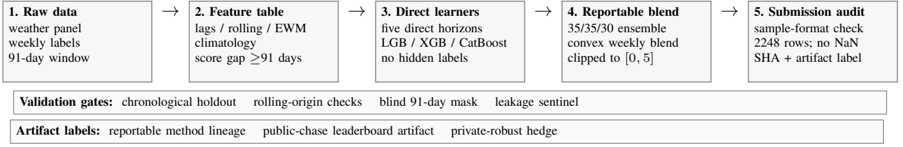
Fig. 1. Method pipeline. Raw weather and sparse weekly score labels are turned into a leakage-aware feature table, then five direct-horizon boosted-tree models are trained for each model family. The final reportable lineage uses a 35/35/30 LightGBM/XGBoost/CatBoost blend, while validation and submission guards keep public-chase and private-hedge artifacts separate from reportable method claims.
