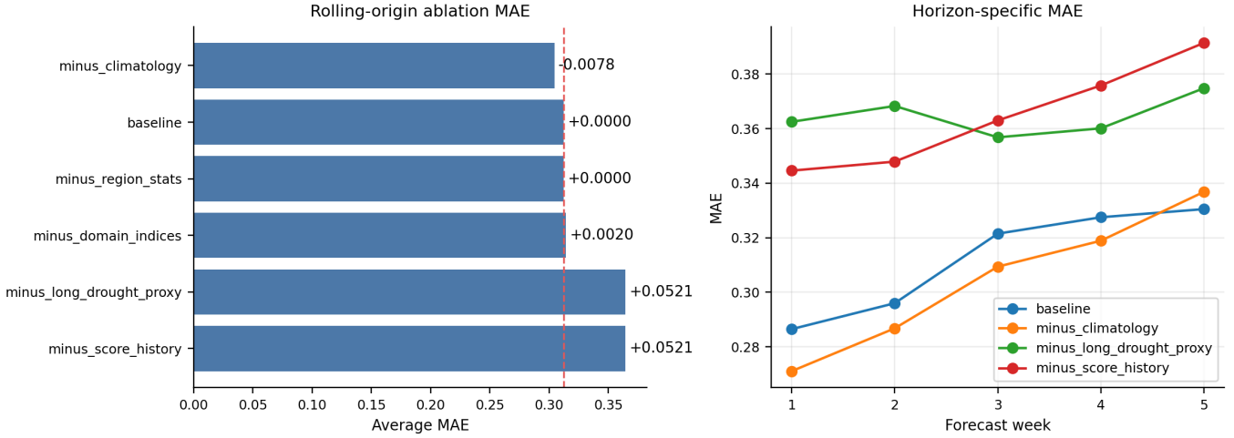
Fig. 4. LightGBM lean tail1095 feature ablation. The left panel compares rolling-origin average MAE against the baseline; the right panel shows how the largest feature removals affect each forecast horizon.
