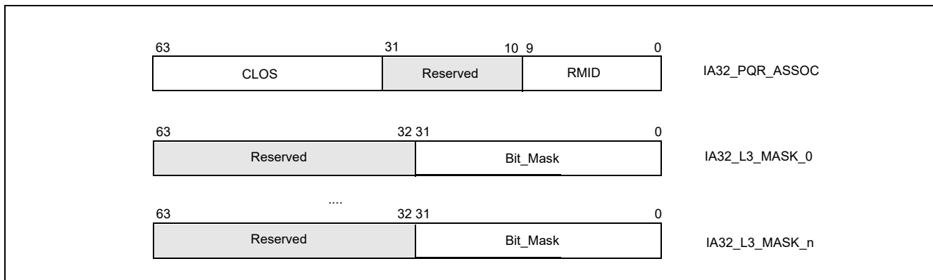
Figure 20-33. IA32_PQR_ASSOC, IA32_L3_MASK_n MSRs
