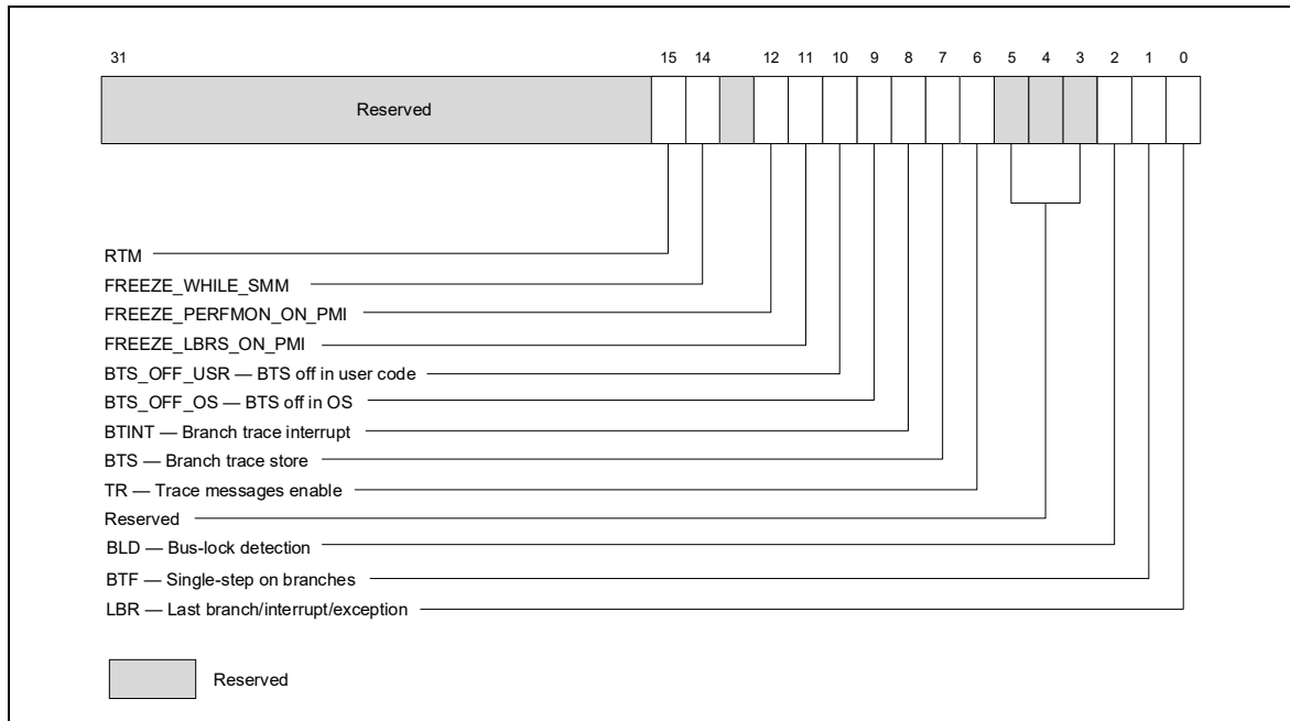
Figure 20-2. IA32_DEBUGCTL MSR for Processors Based on Intel® Core™ Microarchitecture
