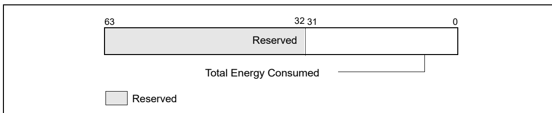
Figure 17-41. MSR_PP0_ENERGY_STATUS/MSR_PP1_ENERGY_STATUS MSR
