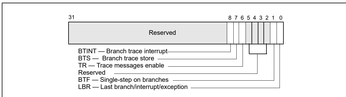
Figure 20-13. IA32_DEBUGCTL MSR for Intel® Core™ Solo and Intel® Core™ Duo Processors
