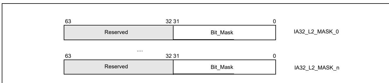
Figure 20-34. IA32_L2_MASK_n MSRs
