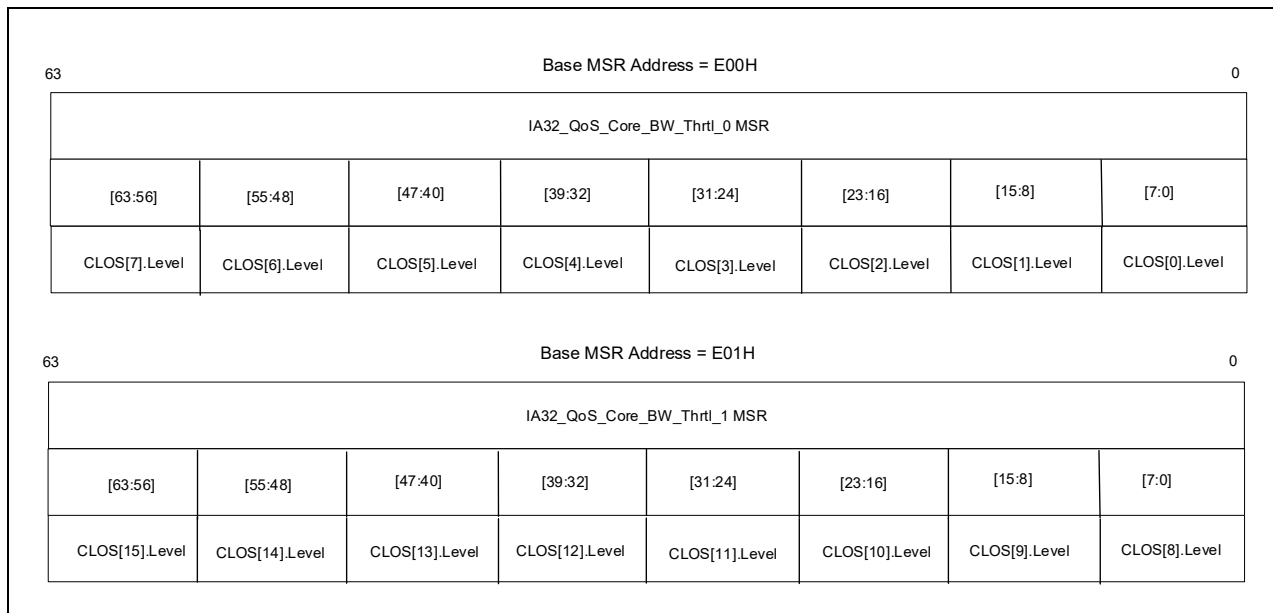
Figure 20-40. IA32_QoS_Core_BW_Thrtl_n MSR Definition
