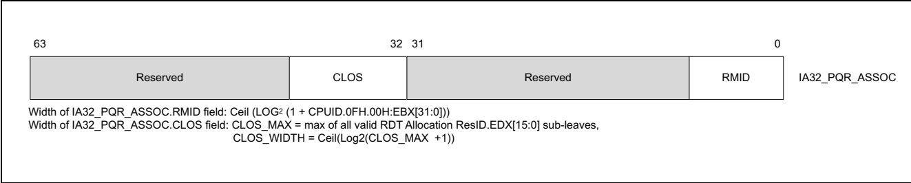
Figure 20-22. IA32_PQR_ASSOC MSR
