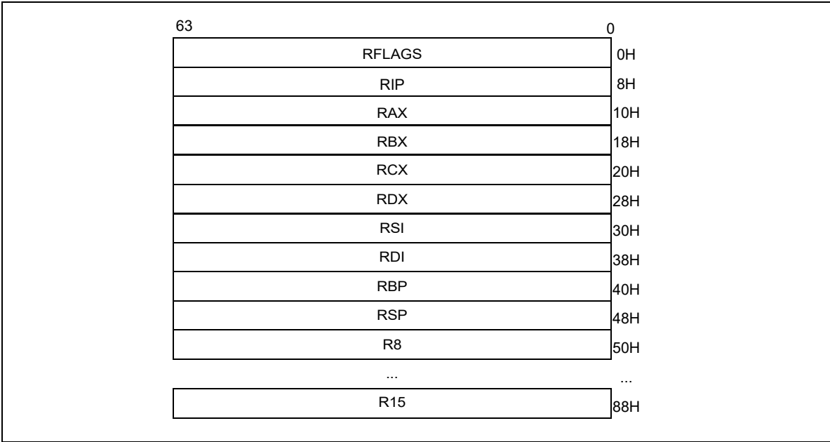
Figure 20-9. 64-bit PEBS Record Format
