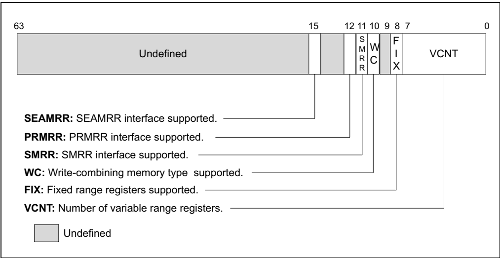
Figure 14-5. IA32_MTRRCAP Register
