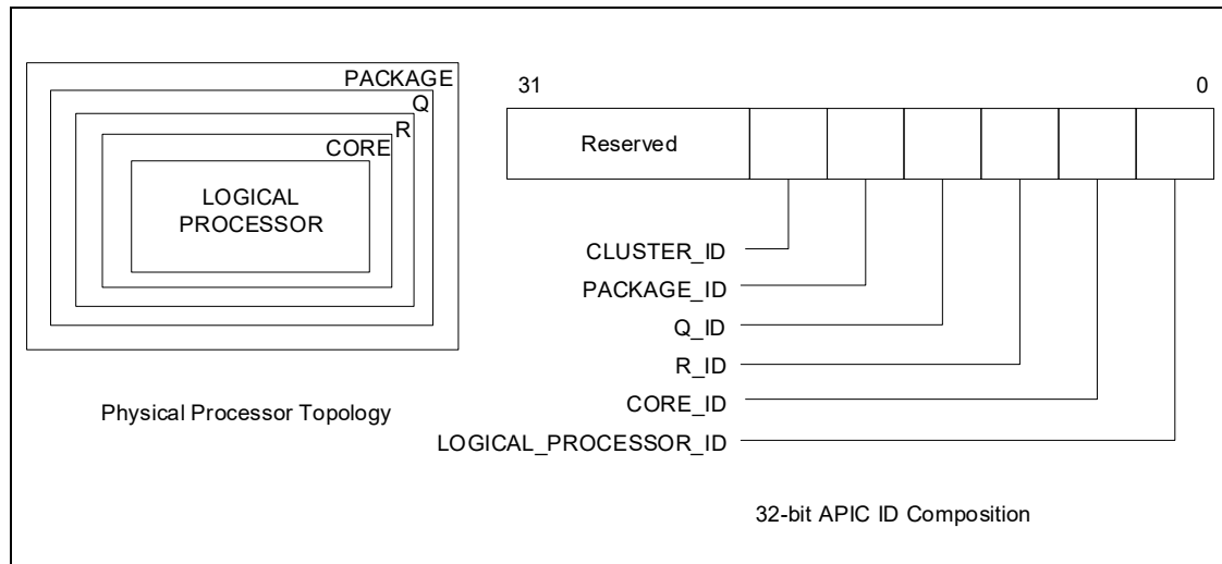
Figure 11-6. Conceptual Six-Domain Topology and 32-bit APIC ID Composition
