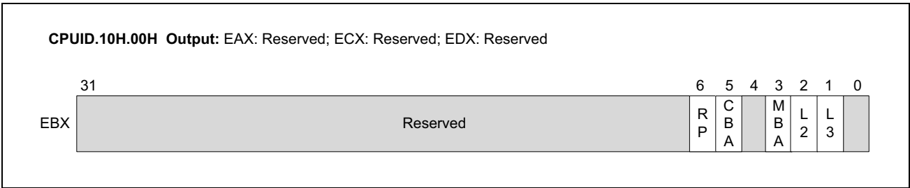
Figure 20-30. CPUID.10H.00H Available Resource Type Identification
