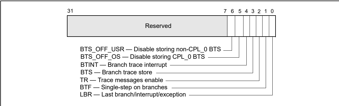
Figure 20-11. MSR_DEBUGCTLA MSR for Pentium 4 and Intel Xeon Processors
