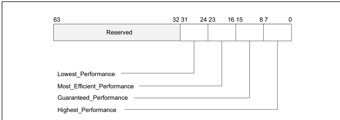
Figure 17-5. IA32_HWP_CAPABILITIES Register
