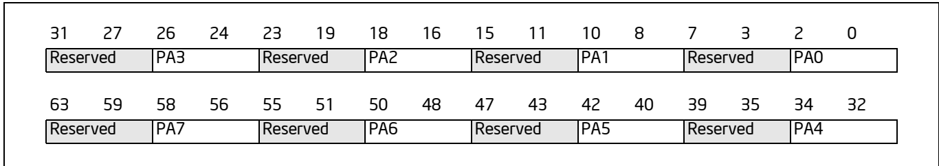
Figure 14-9. IA32_PAT MSR
