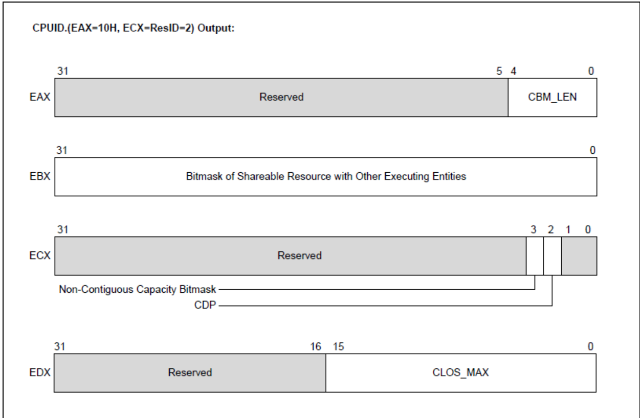
Figure 20-32. L2 Cache Allocation Technology
