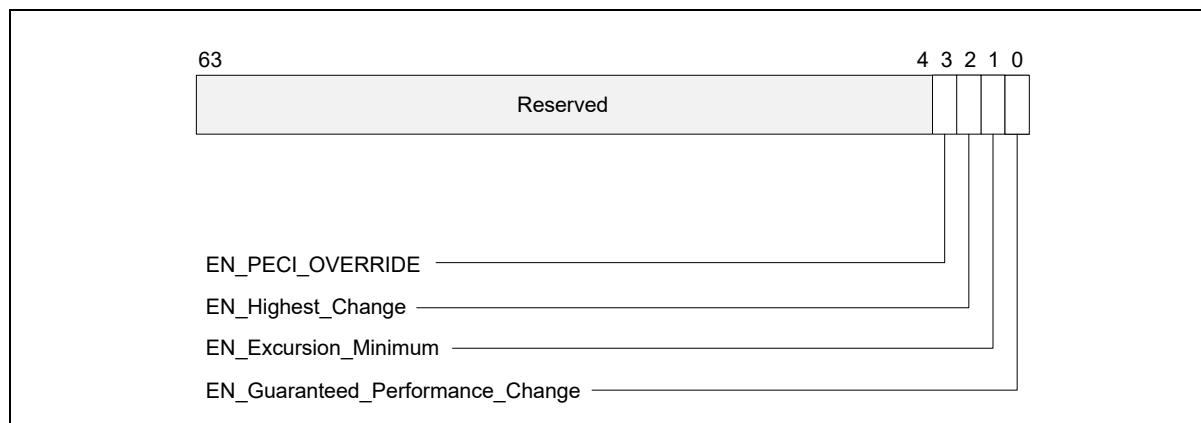
Figure 17-12. IA32_HWP_INTERRUPT MSR
