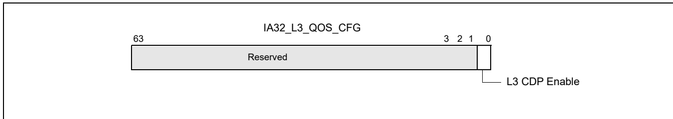
Figure 20-35. Layout of IA32_L3_QOS_CFG
