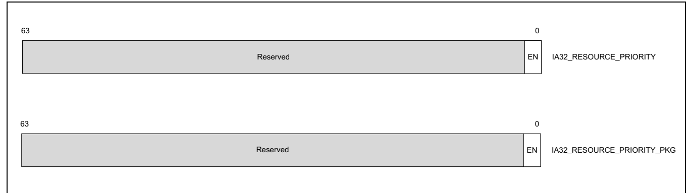
Figure 20-43. IA32_RESOURCE_PRIORITY and IA32_RESOURCE_PRIORITY_PKG Layouts
