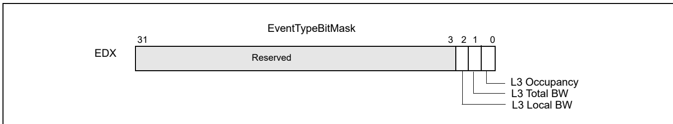
Figure 20-21. L3 Cache Monitoring Capability Enumeration Event Type Bit Vector (CPUID.0FH.01H )
