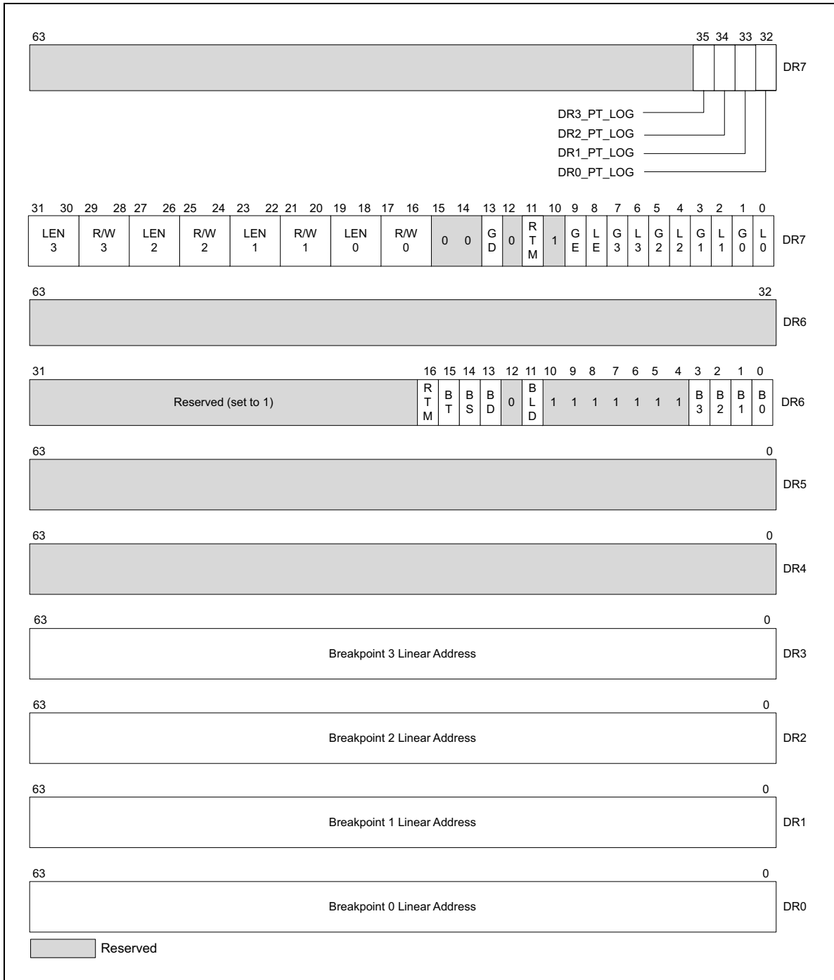
Figure 20-1. Debug Registers
