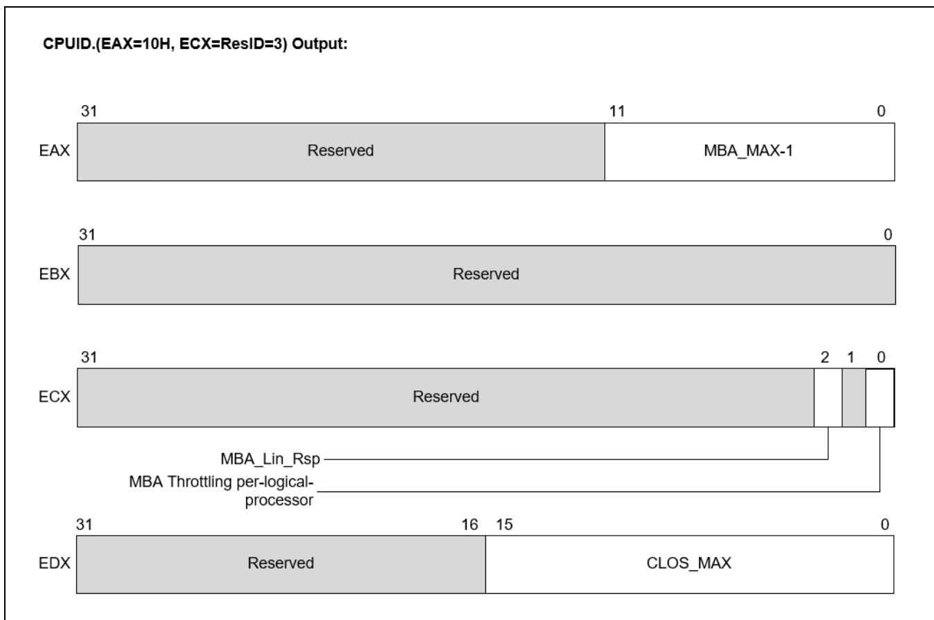
Figure 20-37. CPUID.10H.03H MBA Feature Details Identification
