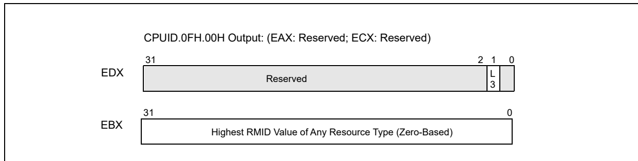
Figure 20-19. CPUID.0FH.00H Monitoring Resource Type Enumeration
