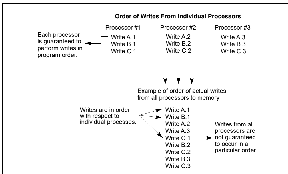
Figure 11-1. Example of Write Ordering in Multiple-Processor Systems
