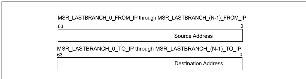
Figure 20-3. 64-bit Address Layout of LBR MSR
