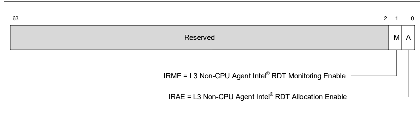
Figure 20-41. Layout of the IA32_L3_IO_RDT_CFG MSR for Enabling Non-CPU Agent Intel® RDT
