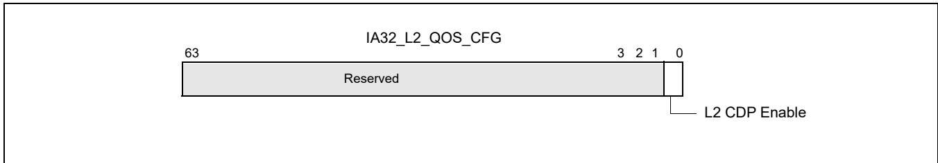
Figure 20-36. Layout of IA32_L2_QOS_CFG
