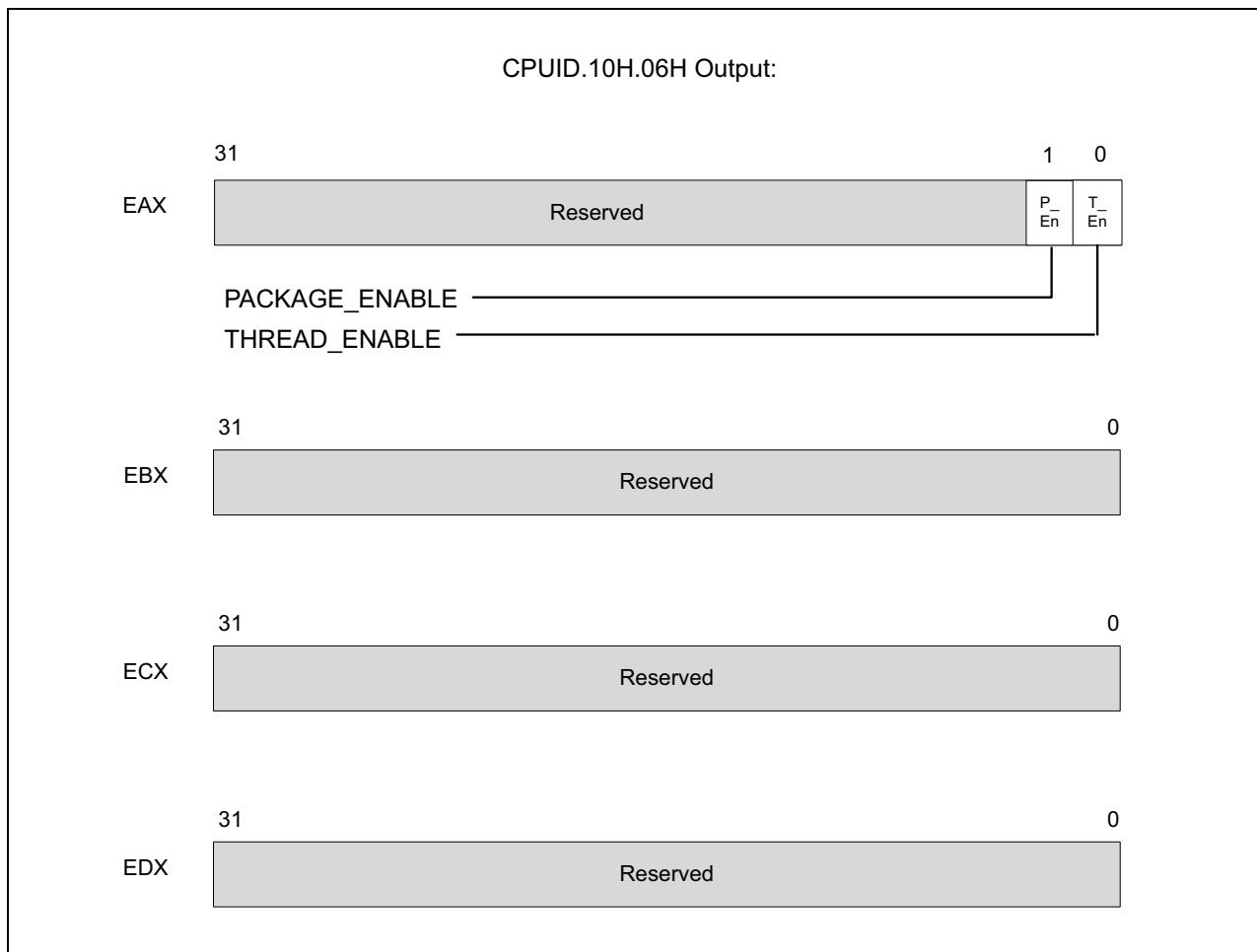
Figure 20-42. CPUID.10H.06H, RP Feature Details Identification
