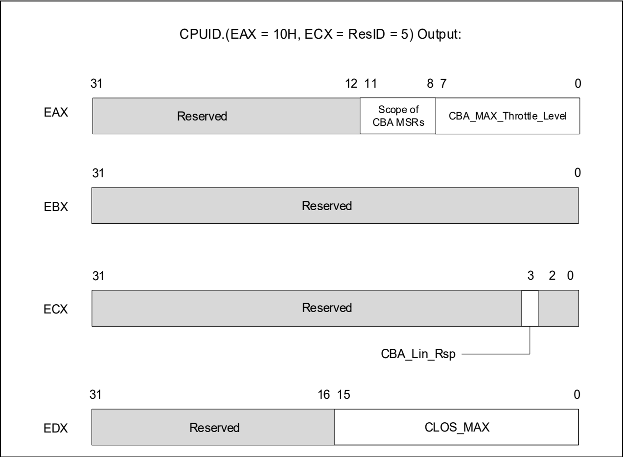
Figure 20-39. CPUID.10H.05H, CBA Feature Details Identification
