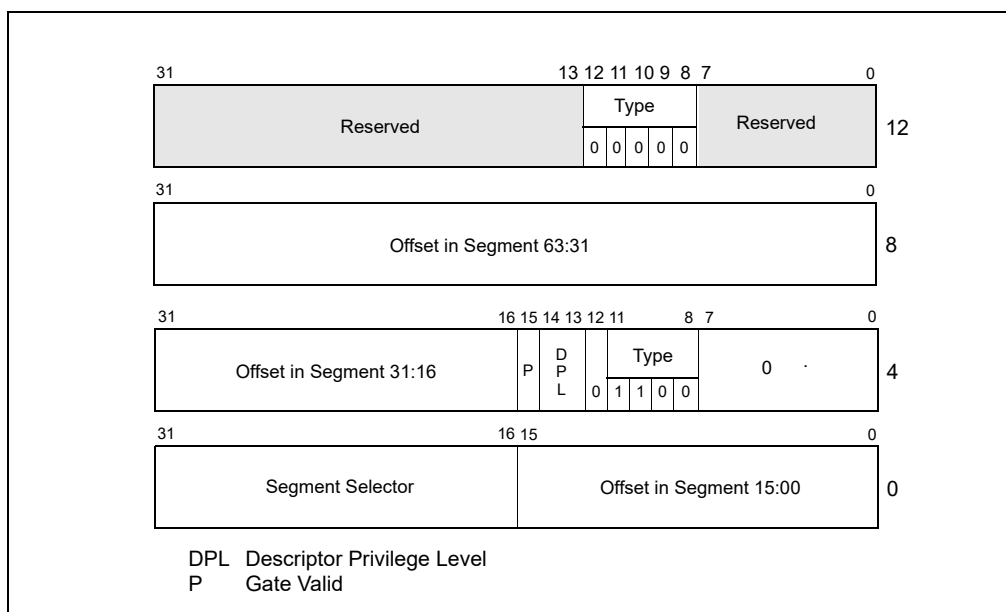
Figure 6-9. Call-Gate Descriptor in IA-32e Mode
