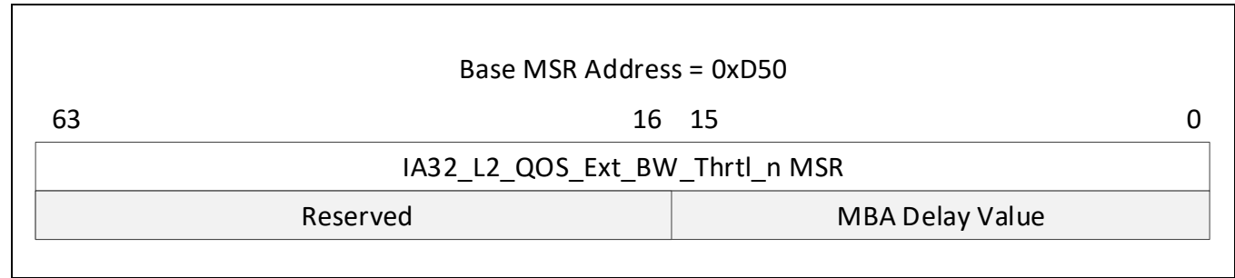
Figure 20-38. IA32_L2_QoS_Ext_BW_Thrtl_n MSR Definition
