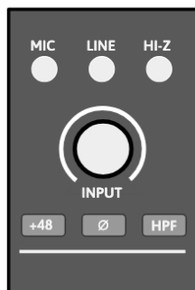
Figure 5: Input section controls, at the top of each channel strip. Input knob controls gain applied by the VCA. The switches at the top select the source type. (MIC switches the input to pass through the PGA2500 preamplifier, and HI-Z switches in a resistor to increase the input impedance to accept direct input instrument signals from things like electric guitar coil pickups. The buttons on the bottom control the +48V phantom power for condenser microphones, phase polarity invert, and high pass filter, respectively. These functions are for the mic preamp only and are built into the PGA2500.
