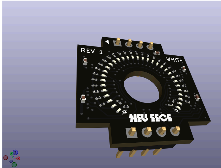
Figure 13: 3D Render of the LED ring, for the small 6mm shaft EC11 encoders, with a 7.5mm diameter hole for that shaft.
