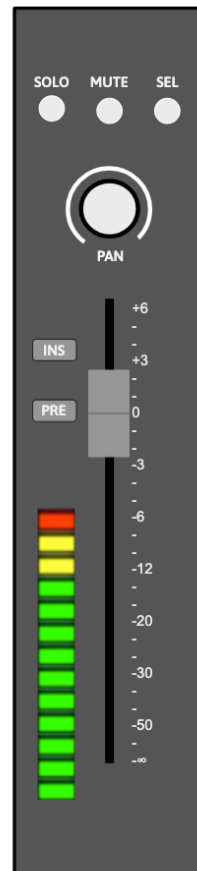
Figure 6: Output section controls, at the bottom of each channel strip. The LED strip is a simple VU meter bar display implemented with a LM3916. The channel fader is shown (See Section 4.6), and the stereo pan(orama) balance control. SOLO mutes all other channels, MUTE mutes this channel, SEL selects the channel for functions like channel grouping or group parameter changes. INS switches the channel effects insert loop, which sends the audio out, to some external processor, and receives it back as a line-level signal. PRE sets the source point for this effects loop to be before the application of the fader and pan VCA gain. (PREfader)
