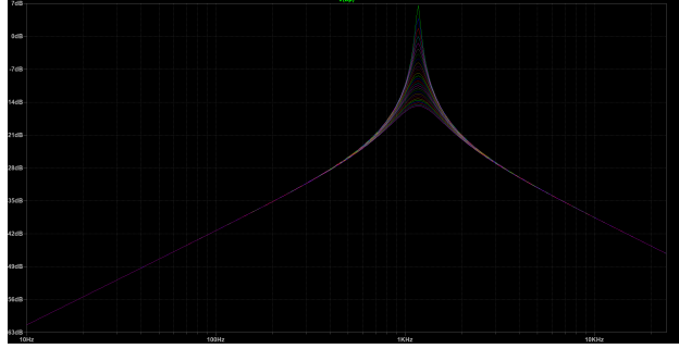
Figure 9: Output frequency response at the band pass output, during a sweep of the Q control voltage from -14V to +14V with 1V steps. Frequency is kept constant.
