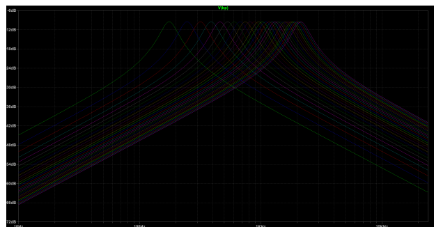
Figure 8: Output frequency response at the band pass output, during a sweep of the frequency control voltage from -14V to +14V with 1V steps. Q is kept constant. Frequency follows the same direction as voltage, so when voltage increases, so does frequency. For the other 3 in other frequency ranges, this circuit may be duplicated and the integration capacitor value changed.
