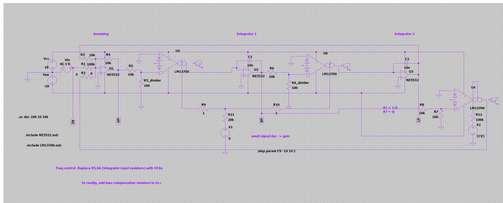
Figure 7: A single variable state filter configured with voltage-controlled center frequency and Q factor, in LTSpice.
