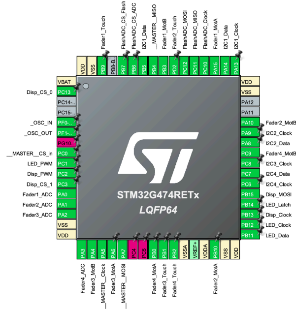
Figure 3: Pin assignments in STM32CubeMX. PG10 is dedicated for reset only. PC4 and 5 are multiplexed with PA2 and 3, respectively on the Nucleo development board, and to reduce complexity, we just avoid PC4 and 5. This is for one bucket of 4 channels. PB8 is the boot mode pin, left open in case we need to tell the microcontroller to boot from the external SPI flash chip (if the firmware does not fit on internal flash)
