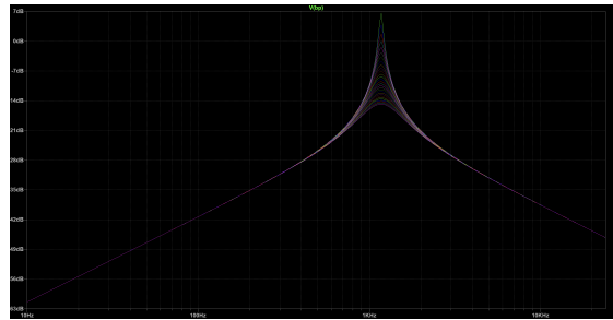
Figure 8: Output frequency response at the band pass output, during a sweep of the Q control voltage from -14V to +14V with 1V steps. Frequency is kept constant.
