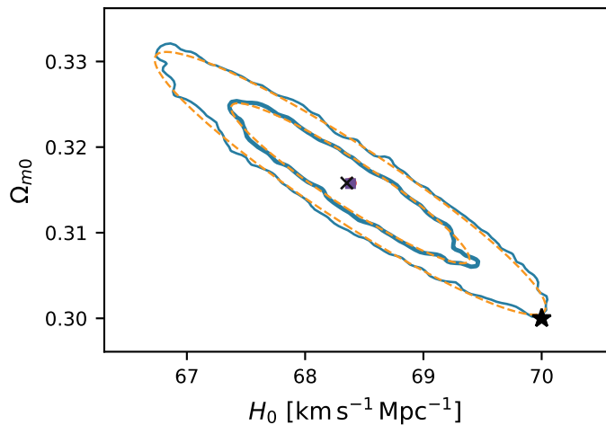
N100-98 largest normalized H_0 -- \Omega_{m0} displacement
