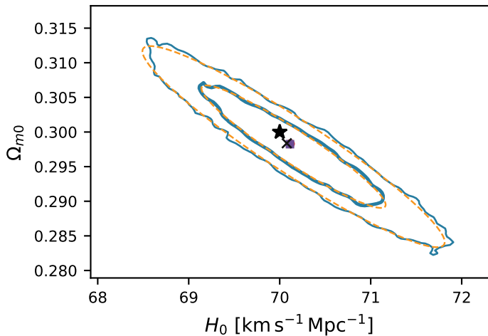
N100-41 closest to generating cosmology
