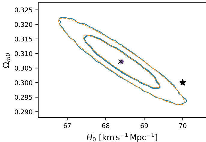
N100-65 largest \Delta\chi^2_{\text{LR}}
