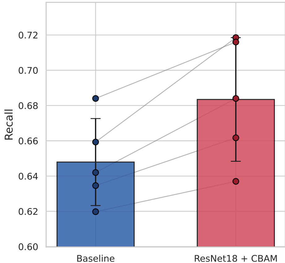
Recall Comparison
