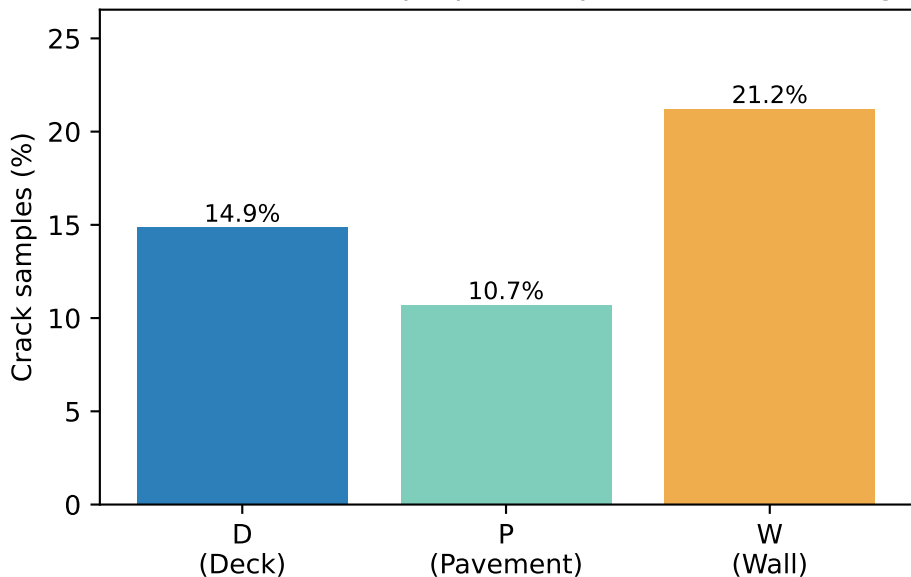
Class balance: crack proportion per structural category
