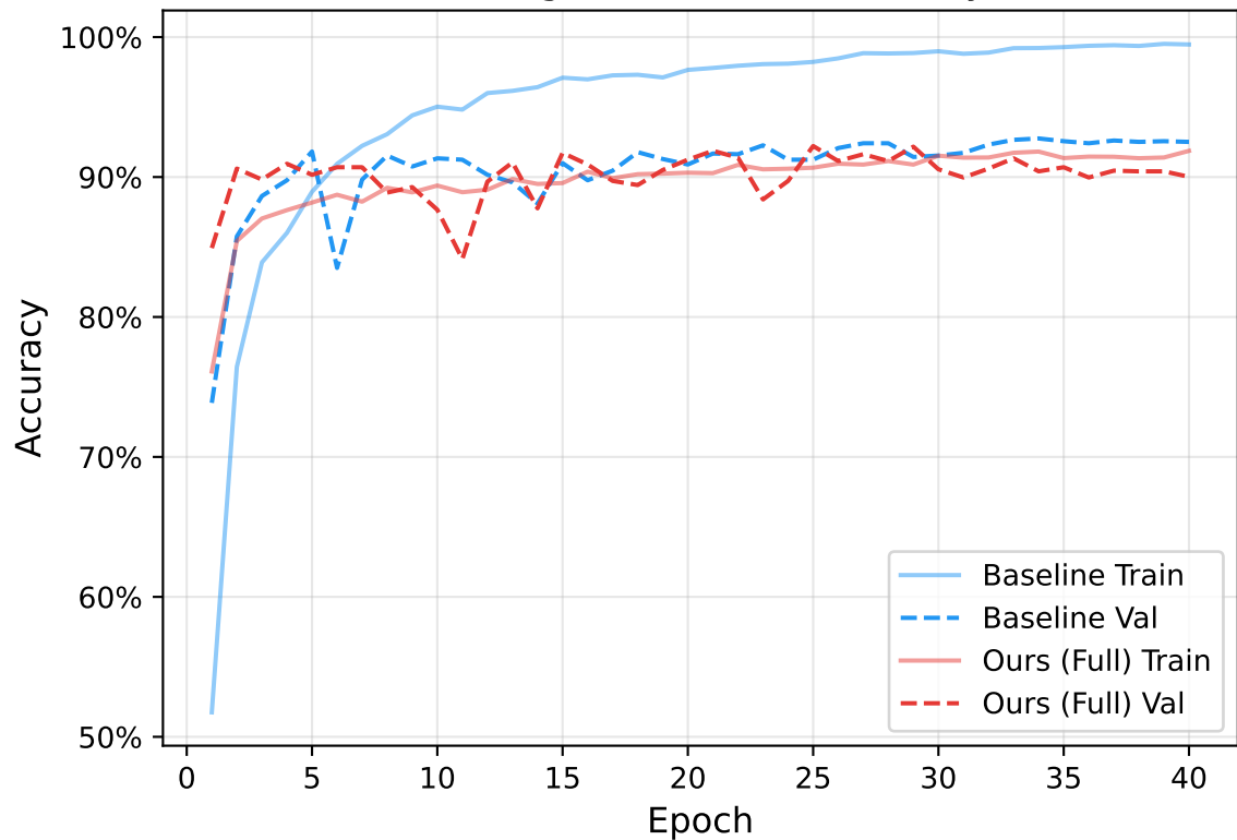
Training &amp; Validation Accuracy
