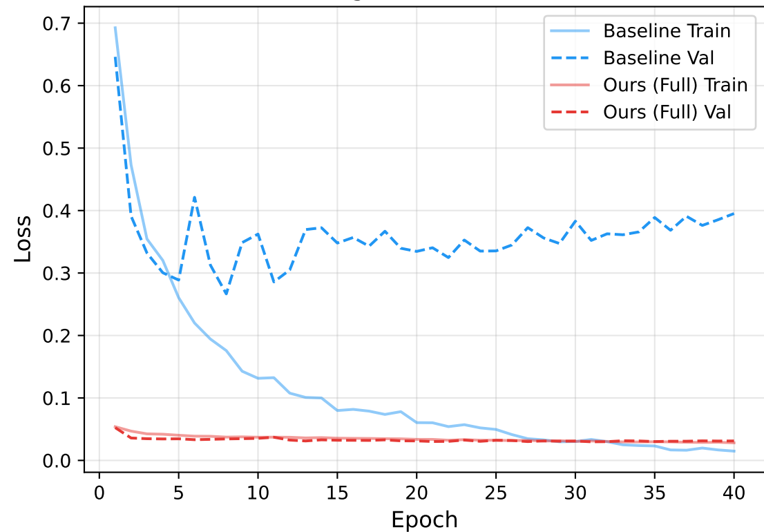
Training &amp; Validation Loss
