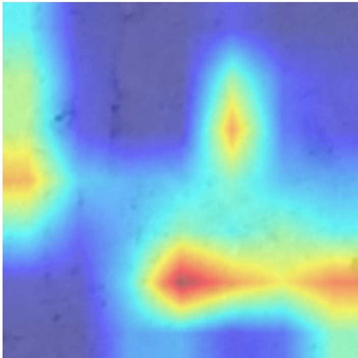
Ours (resnet18+CBAM)
