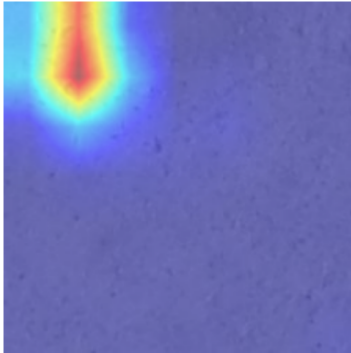
Baseline (resnet18)
