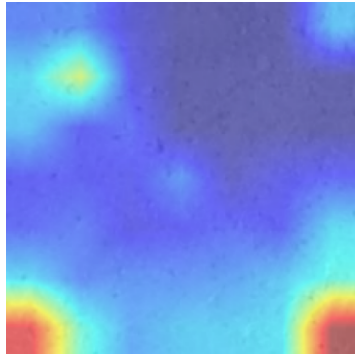
Ours (resnet18+CBAM)
