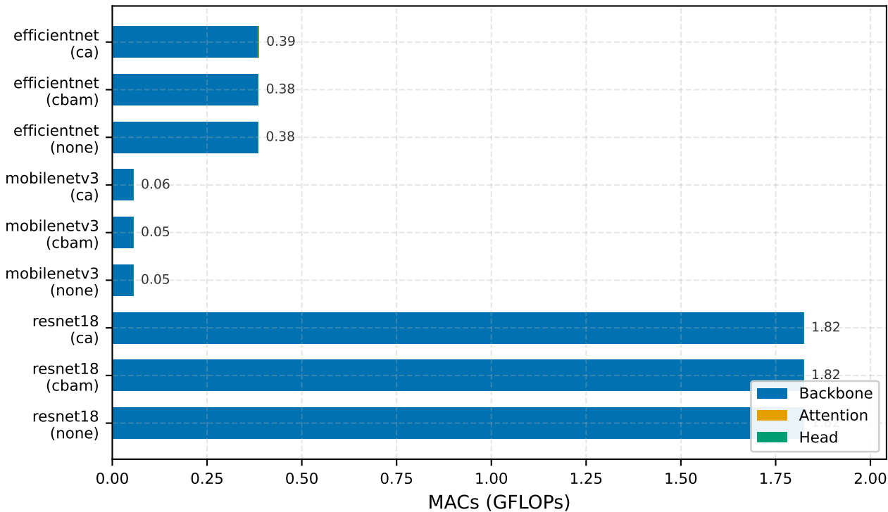
MACs by module (single 224×224 forward, thop convention)
