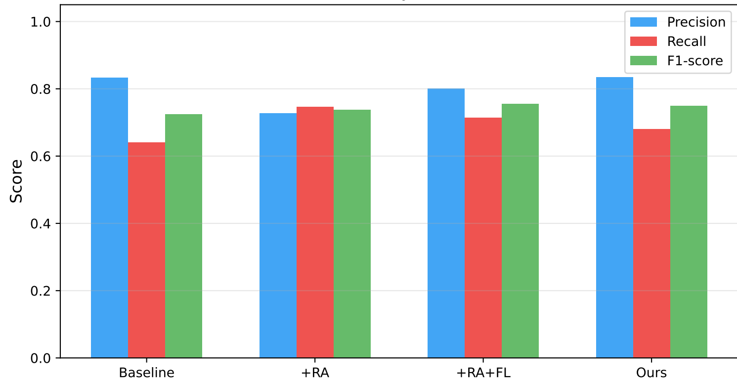
Ablation Study (ResNet18)
