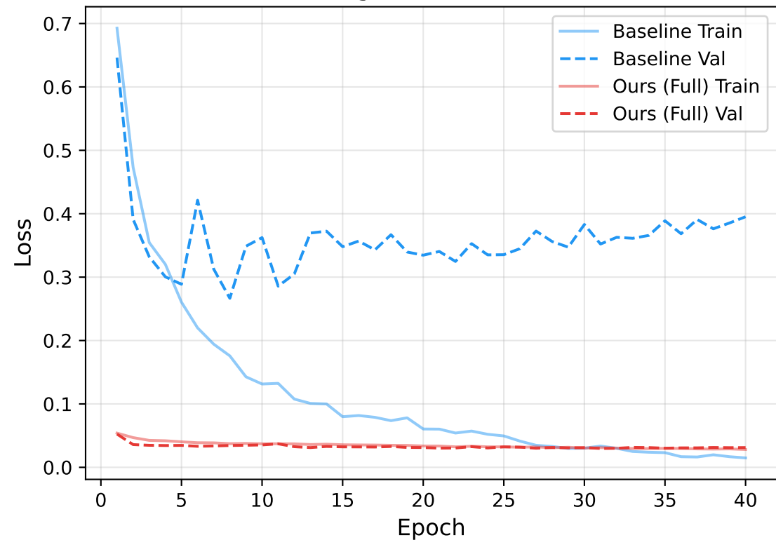
Training & Validation Loss
