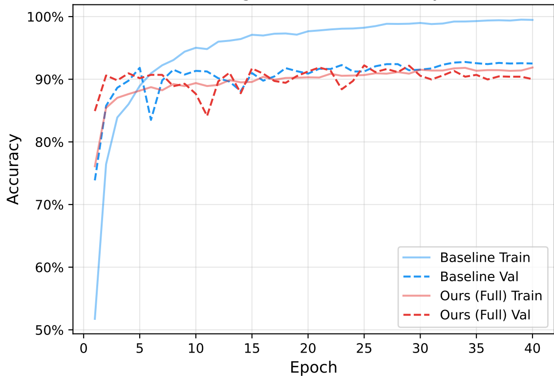
Training & Validation Accuracy
