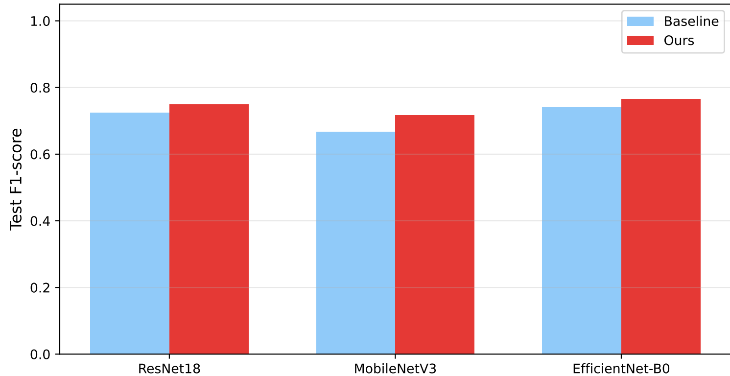
Cross-backbone: baseline vs full method
