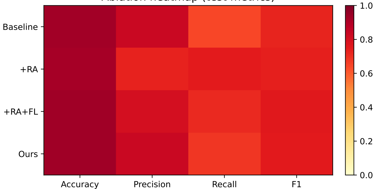
Ablation heatmap (test metrics)
